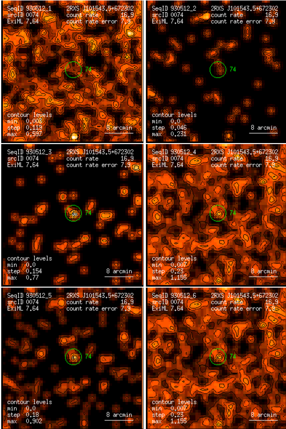
Figure 74: RASS 930512: detection 0074: band rate images, Gaussian filter: (1) PSPC channels 11 – 41, (2) 52 – 90, (3) 91 – 201, (4) 11 – 235, (5) 52 – 201, (6) 11 – 201. Broad band rates in counts/ks. Band rate contour levels in counts/ks/arcmin 2 .
