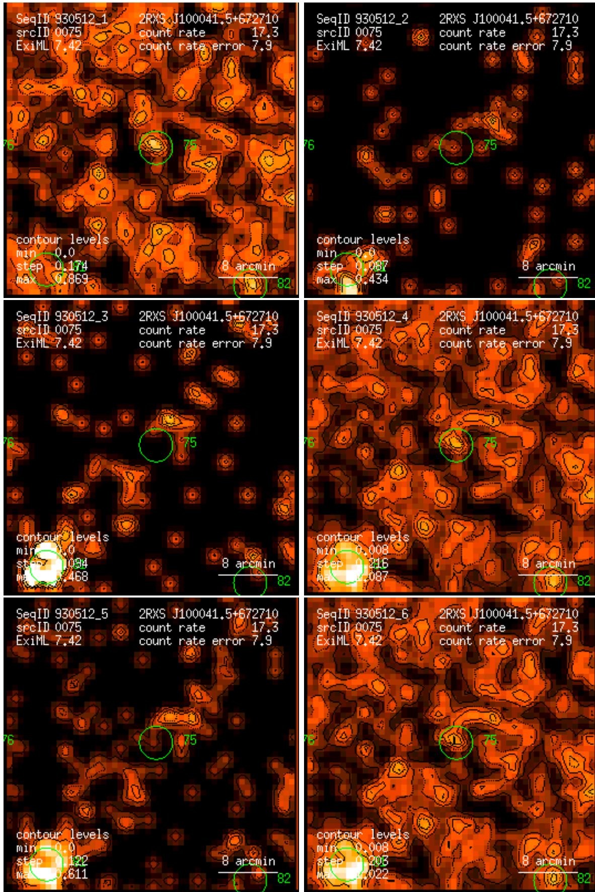
Figure 75: RASS 930512: detection 0075: band rate images, Gaussian filter: (1) PSPC channels 11 – 41, (2) 52 – 90, (3) 91 – 201, (4) 11 – 235, (5) 52 – 201, (6) 11 – 201. Broad band rates in counts/ks. Band rate contour levels in counts/ks/arcmin 2 .
