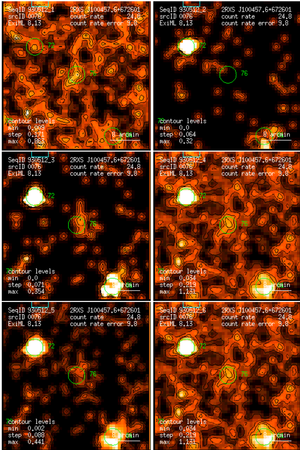
Figure 76: RASS 930512: detection 0076: band rate images, Gaussian filter: (1) PSPC channels 11 – 41, (2) 52 – 90, (3) 91 – 201, (4) 11 – 235, (5) 52 – 201, (6) 11 – 201. Broad band rates in counts/ks. Band rate contour levels in counts/ks/arcmin 2 .
