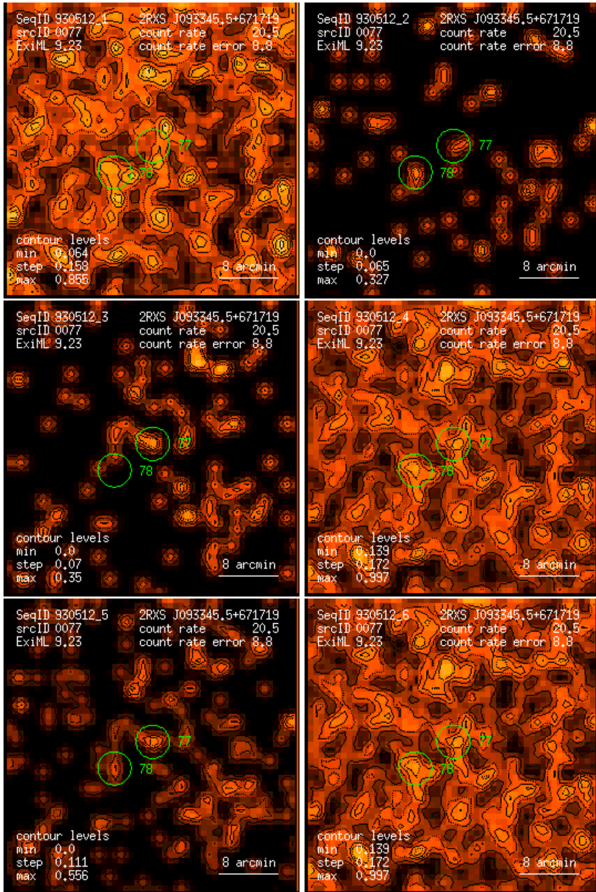
Figure 77: RASS 930512: detection 0077: band rate images, Gaussian filter: (1) PSPC channels 11 – 41, (2) 52 – 90, (3) 91 – 201, (4) 11 – 235, (5) 52 – 201, (6) 11 – 201. Broad band rates in counts/ks. Band rate contour levels in counts/ks/arcmin 2 .
