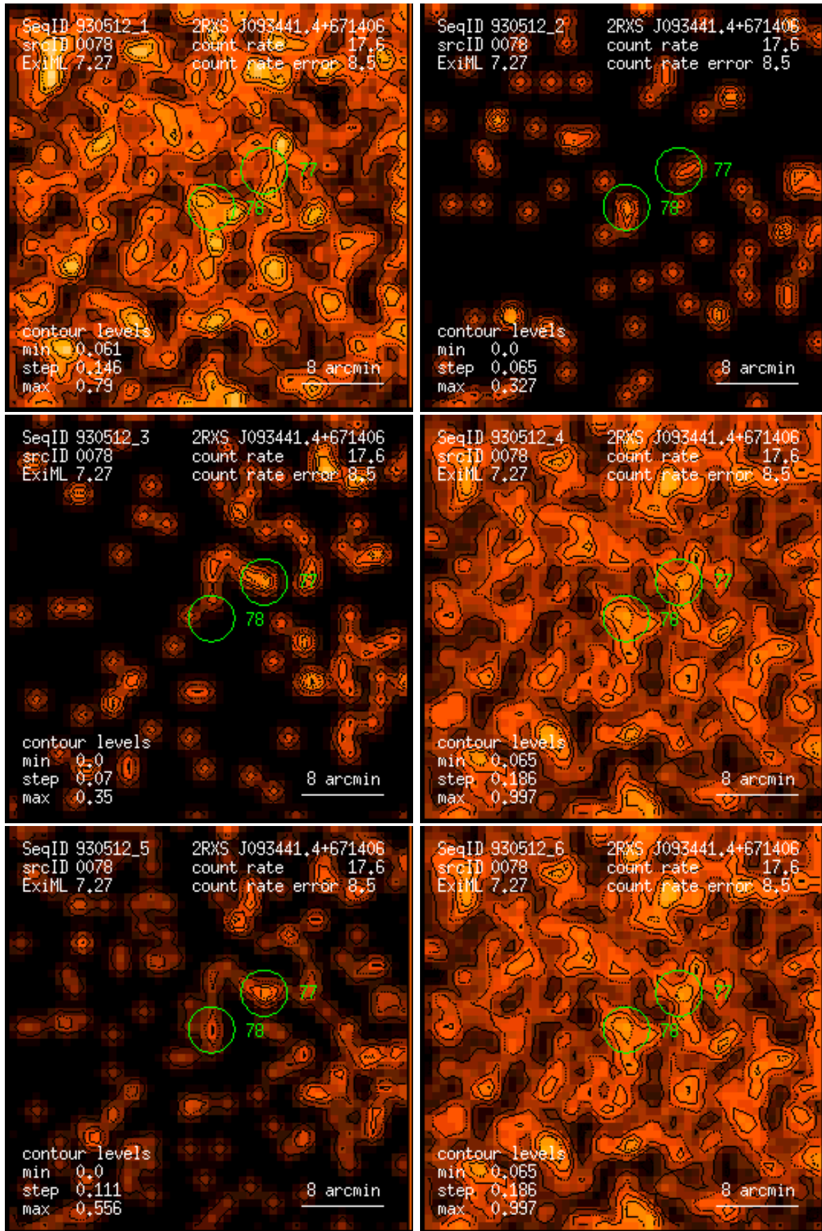
Figure 78: RASS 930512: detection 0078: band rate images, Gaussian filter: (1) PSPC channels 11 – 41, (2) 52 – 90, (3) 91 – 201, (4) 11 – 235, (5) 52 – 201, (6) 11 – 201. Broad band rates in counts/ks. Band rate contour levels in counts/ks/arcmin 2 .
