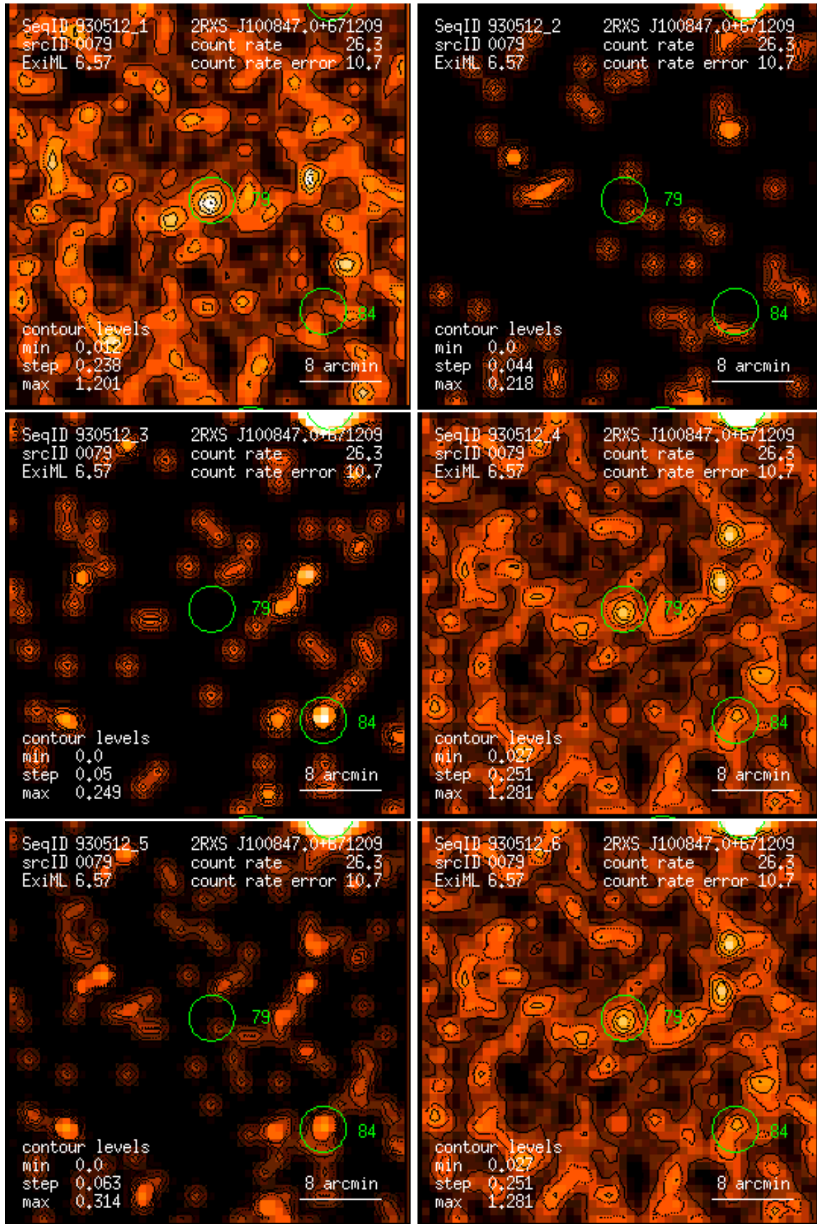
Figure 79: RASS 930512: detection 0079: band rate images, Gaussian filter: (1) PSPC channels 11 – 41, (2) 52 – 90, (3) 91 – 201, (4) 11 – 235, (5) 52 – 201, (6) 11 – 201. Broad band rates in counts/ks. Band rate contour levels in counts/ks/arcmin 2 .
