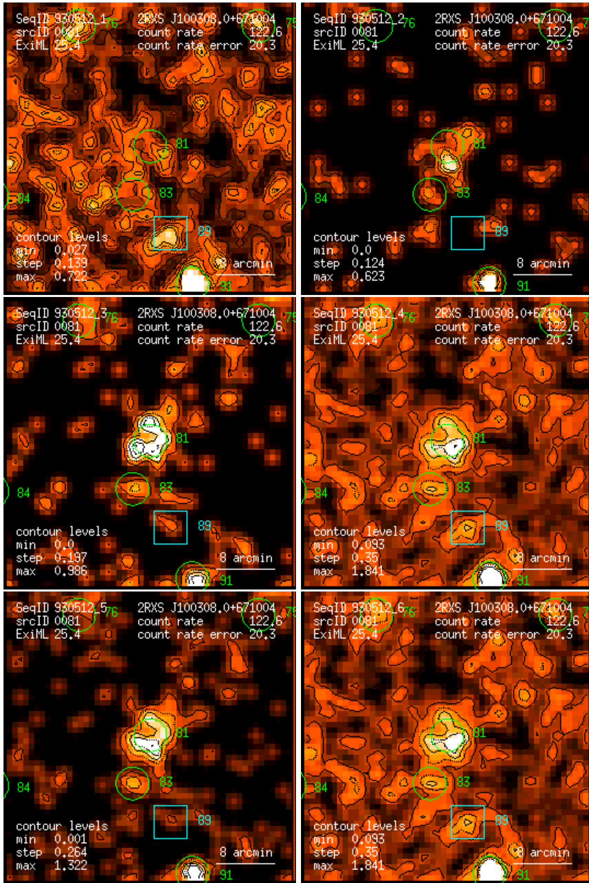
Figure 81: RASS 930512: detection 0081: band rate images, Gaussian filter: (1) PSPC channels 11 – 41, (2) 52 – 90, (3) 91 – 201, (4) 11 – 235, (5) 52 – 201, (6) 11 – 201. Broad band rates in counts/ks. Band rate contour levels in counts/ks/arcmin 2 .
