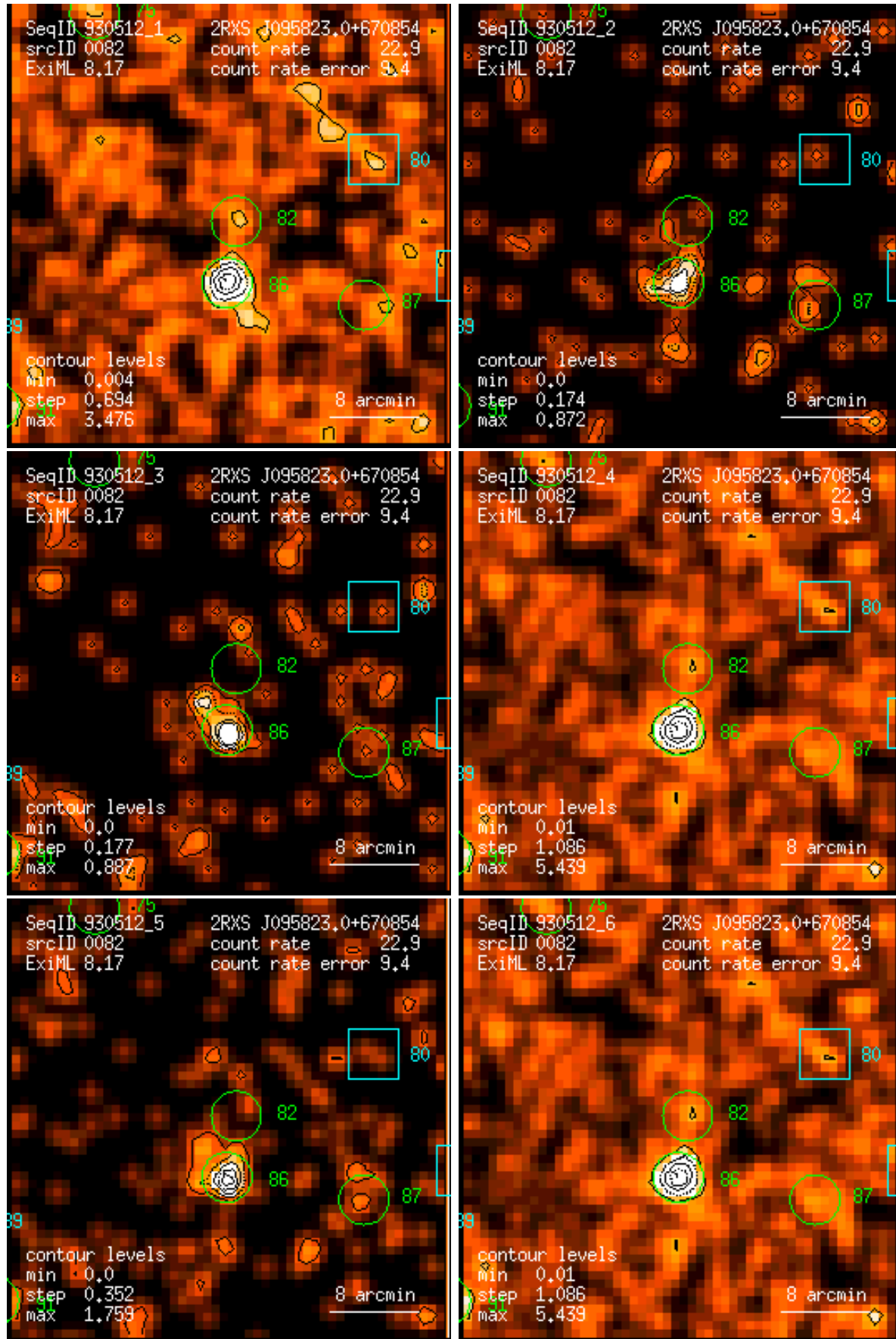
Figure 82: RASS 930512: detection 0082: band rate images, Gaussian filter: (1) PSPC channels 11 – 41, (2) 52 – 90, (3) 91 – 201, (4) 11 – 235, (5) 52 – 201, (6) 11 – 201. Broad band rates in counts/ks. Band rate contour levels in counts/ks/arcmin 2 .
