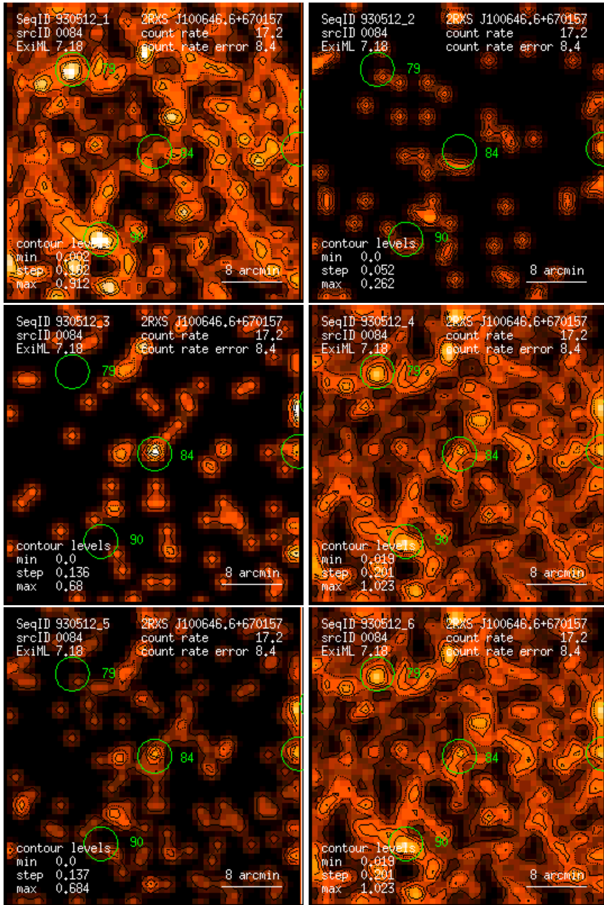
Figure 84: RASS 930512: detection 0084: band rate images, Gaussian filter: (1) PSPC channels 11 – 41, (2) 52 – 90, (3) 91 – 201, (4) 11 – 235, (5) 52 – 201, (6) 11 – 201. Broad band rates in counts/ks. Band rate contour levels in counts/ks/arcmin 2 .
