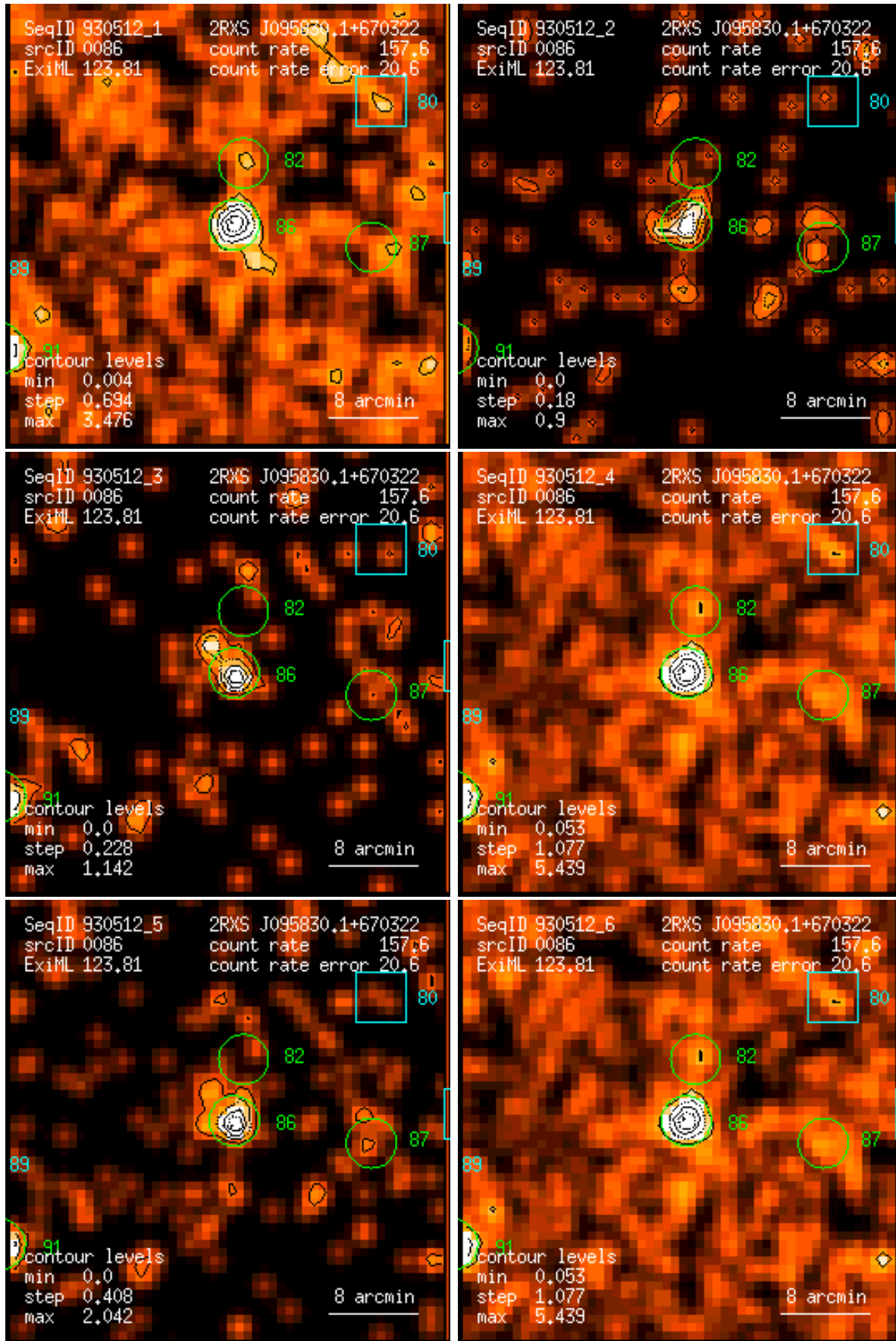
Figure 86: RASS 930512: detection 0086: band rate images, Gaussian filter: (1) PSPC channels 11 – 41, (2) 52 – 90, (3) 91 – 201, (4) 11 – 235, (5) 52 – 201, (6) 11 – 201. Broad band rates in counts/ks. Band rate contour levels in counts/ks/arcmin 2 .
