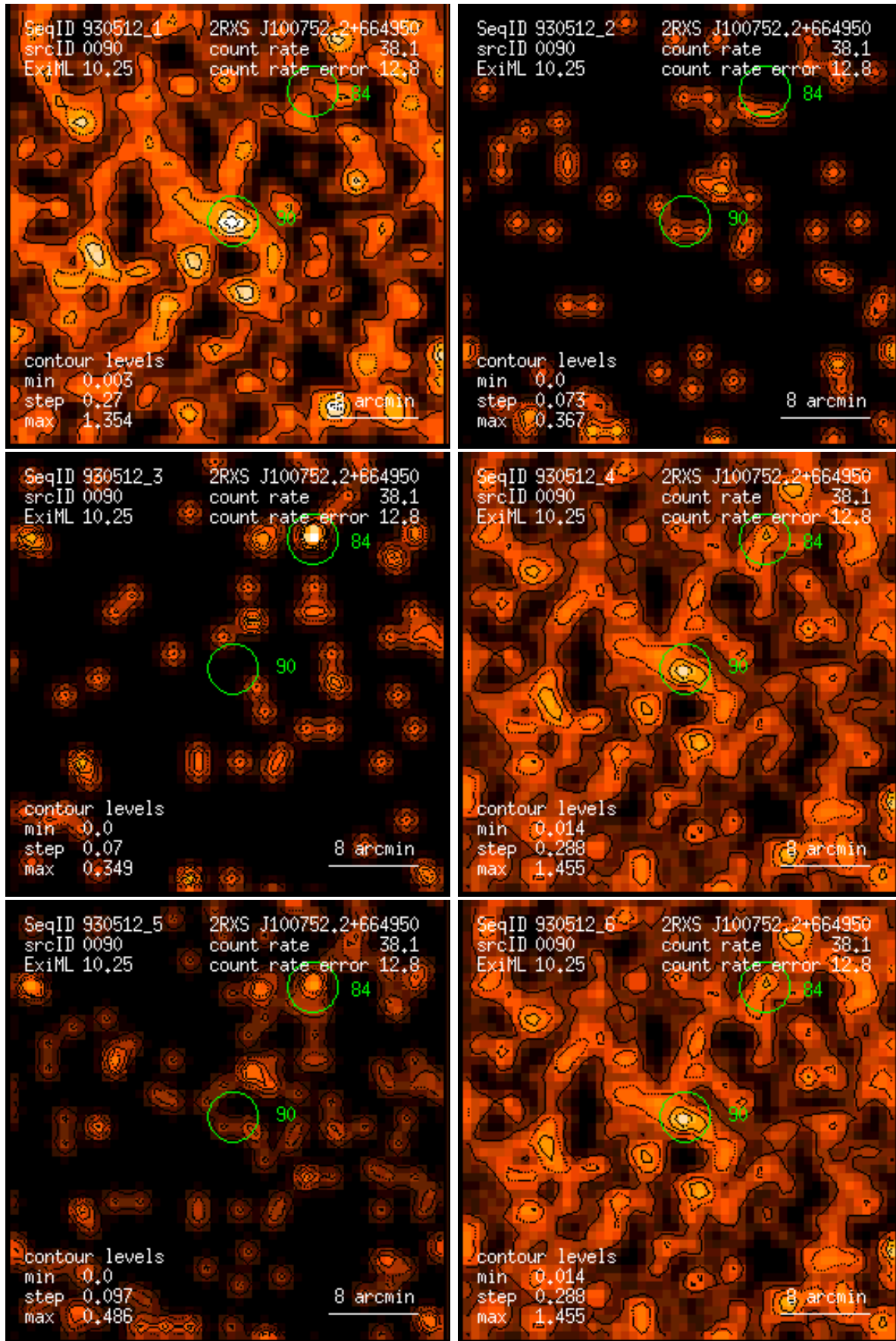
Figure 90: RASS 930512: detection 0090: band rate images, Gaussian filter: (1) PSPC channels 11 – 41, (2) 52 – 90, (3) 91 – 201, (4) 11 – 235, (5) 52 – 201, (6) 11 – 201. Broad band rates in counts/ks. Band rate contour levels in counts/ks/arcmin 2 .
