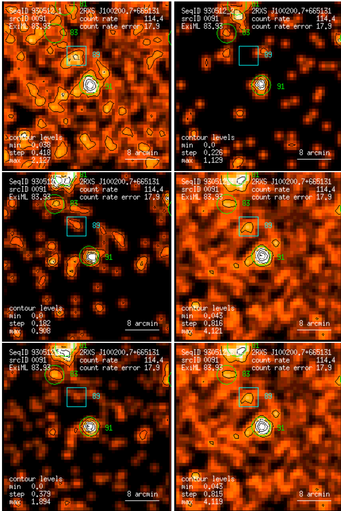
Figure 91: RASS 930512: detection 0091: band rate images, Gaussian filter: (1) PSPC channels 11 – 41, (2) 52 – 90, (3) 91 – 201, (4) 11 – 235, (5) 52 – 201, (6) 11 – 201. Broad band rates in counts/ks. Band rate contour levels in counts/ks/arcmin 2 .
