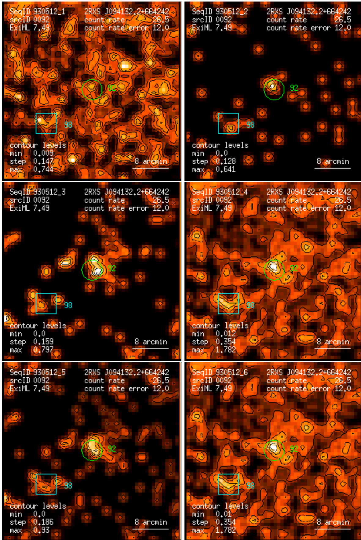
Figure 92: RASS 930512: detection 0092: band rate images, Gaussian filter: (1) PSPC channels 11 – 41, (2) 52 – 90, (3) 91 – 201, (4) 11 – 235, (5) 52 – 201, (6) 11 – 201. Broad band rates in counts/ks. Band rate contour levels in counts/ks/arcmin 2 .
