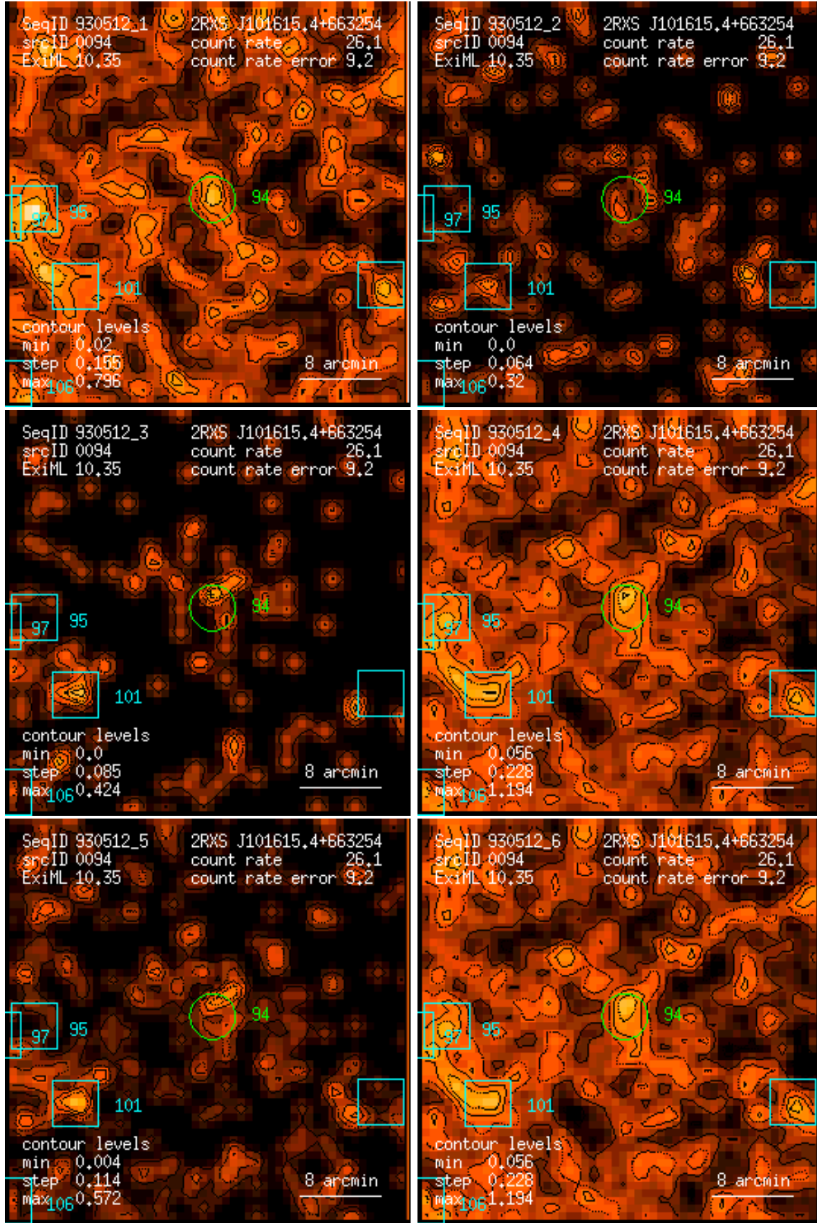
Figure 94: RASS 930512: detection 0094: band rate images, Gaussian filter: (1) PSPC channels 11 – 41, (2) 52 – 90, (3) 91 – 201, (4) 11 – 235, (5) 52 – 201, (6) 11 – 201. Broad band rates in counts/ks. Band rate contour levels in counts/ks/arcmin 2 .
