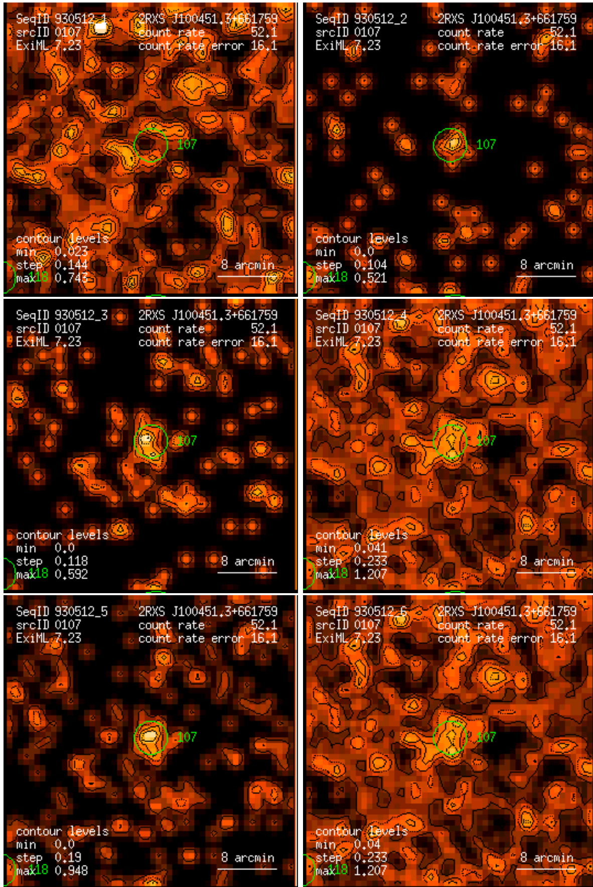
Figure 107: RASS 930512: detection 0107: band rate images, Gaussian filter: (1) PSPC channels 11 – 41, (2) 52 – 90, (3) 91 – 201, (4) 11 – 235, (5) 52 – 201, (6) 11 – 201. Broad band rates in counts/ks. Band rate contour levels in counts/ks/arcmin 2 .
