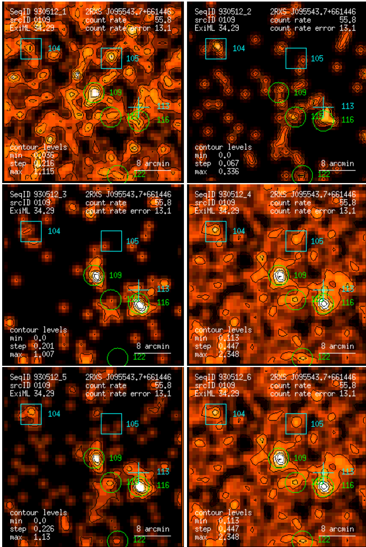
Figure 109: RASS 930512: detection 0109: band rate images, Gaussian filter: (1) PSPC channels 11 – 41, (2) 52 – 90, (3) 91 – 201, (4) 11 – 235, (5) 52 – 201, (6) 11 – 201. Broad band rates in counts/ks. Band rate contour levels in counts/ks/arcmin 2 .
