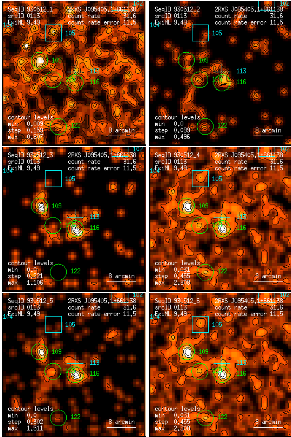
Figure 113: RASS 930512: detection 0113: band rate images, Gaussian filter: (1) PSPC channels 11 – 41, (2) 52 – 90, (3) 91 – 201, (4) 11 – 235, (5) 52 – 201, (6) 11 – 201. Broad band rates in counts/ks. Band rate contour levels in counts/ks/arcmin 2 .
