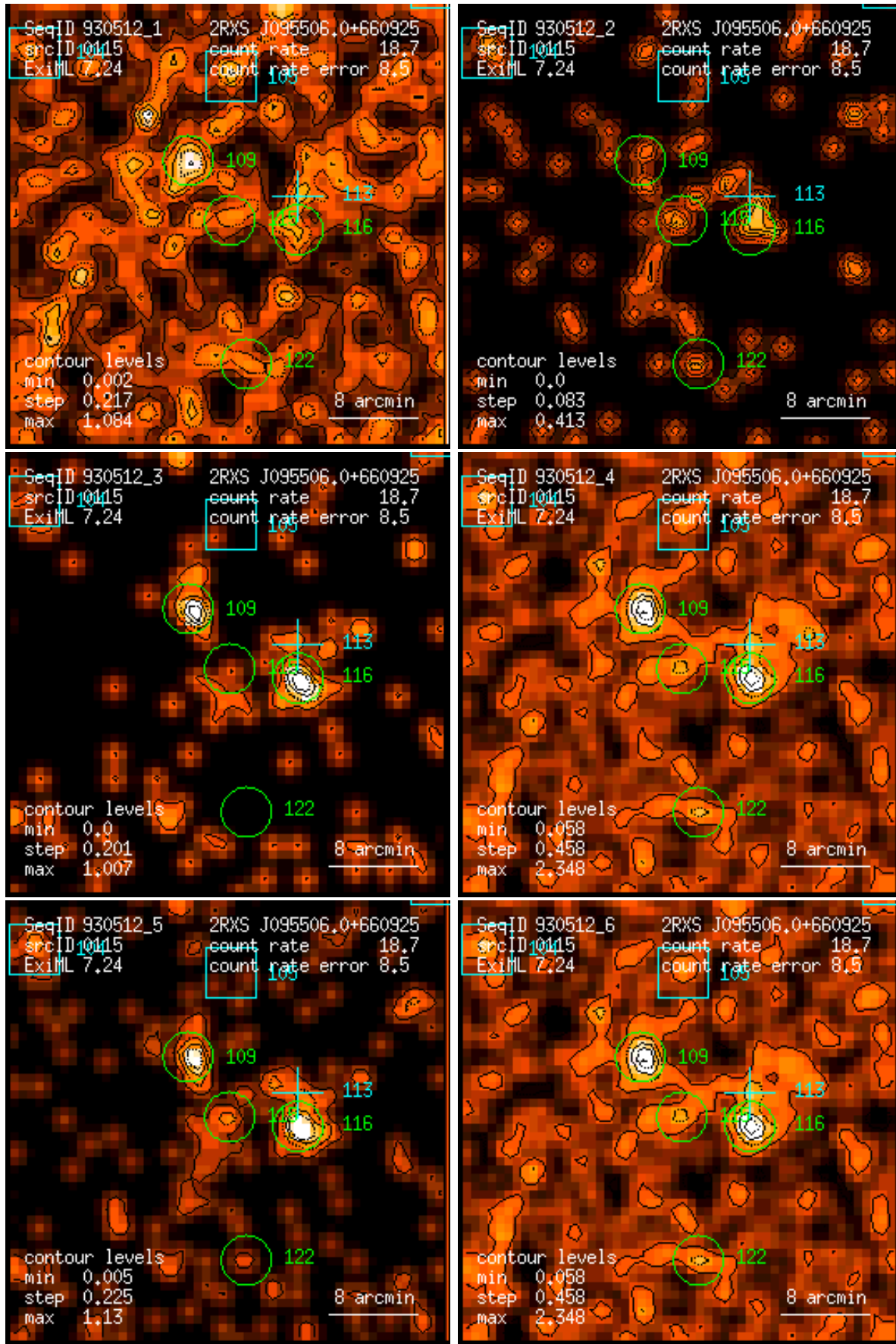
Figure 115: RASS 930512: detection 0115: band rate images, Gaussian filter: (1) PSPC channels 11 – 41, (2) 52 – 90, (3) 91 – 201, (4) 11 – 235, (5) 52 – 201, (6) 11 – 201. Broad band rates in counts/ks. Band rate contour levels in counts/ks/arcmin 2 .
