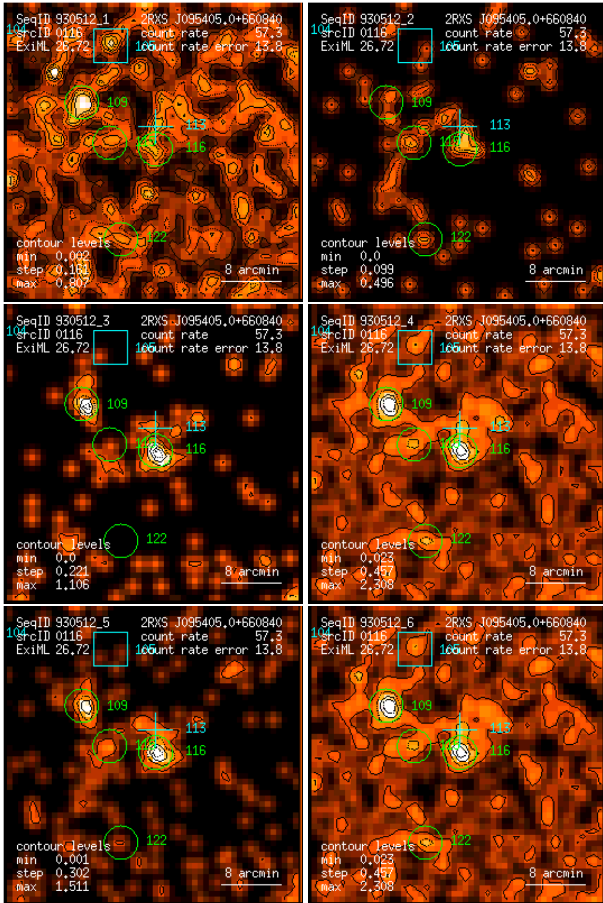
Figure 116: RASS 930512: detection 0116: band rate images, Gaussian filter: (1) PSPC channels 11 – 41, (2) 52 – 90, (3) 91 – 201, (4) 11 – 235, (5) 52 – 201, (6) 11 – 201. Broad band rates in counts/ks. Band rate contour levels in counts/ks/arcmin 2 .
