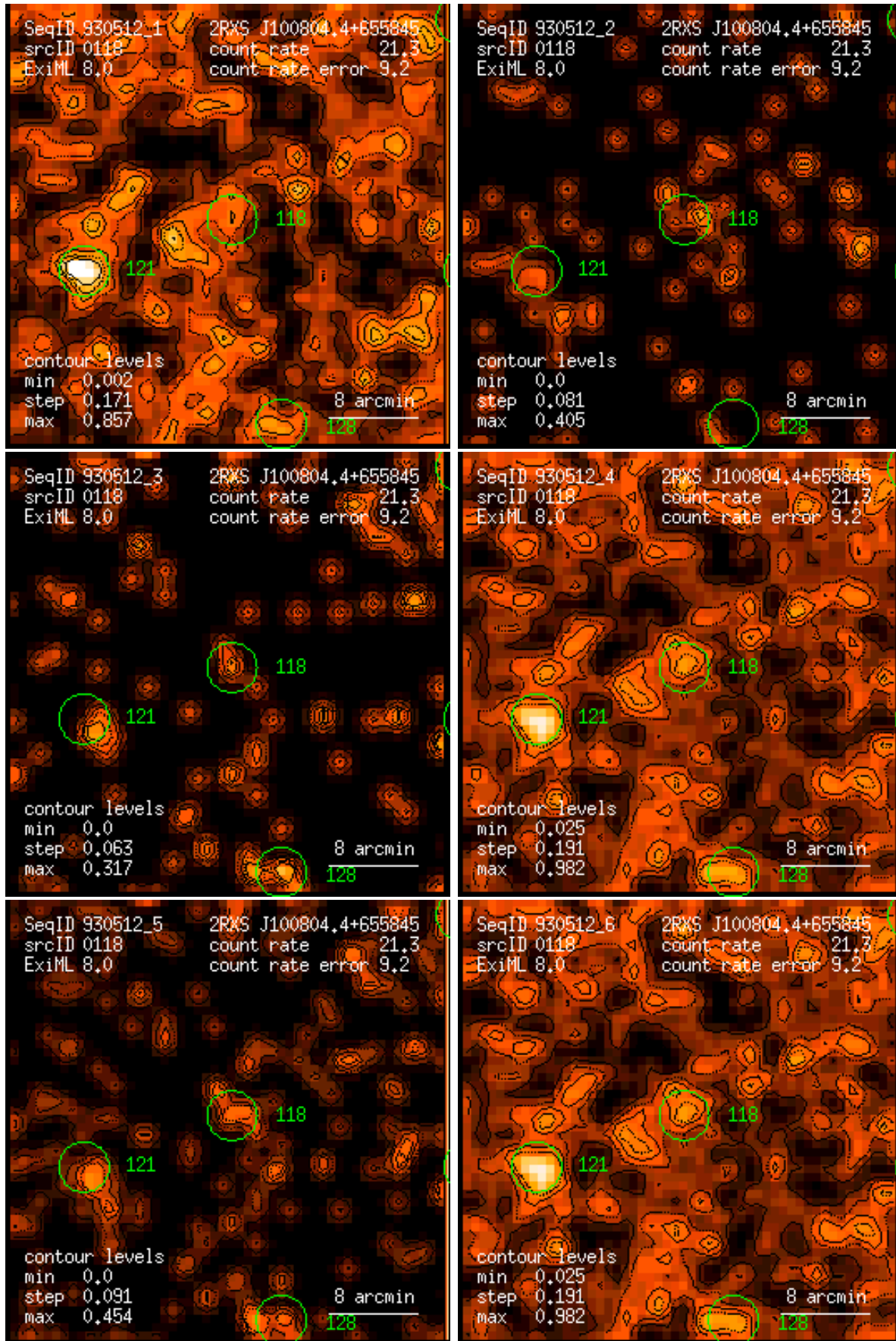
Figure 118: RASS 930512: detection 0118: band rate images, Gaussian filter: (1) PSPC channels 11 – 41, (2) 52 – 90, (3) 91 – 201, (4) 11 – 235, (5) 52 – 201, (6) 11 – 201. Broad band rates in counts/ks. Band rate contour levels in counts/ks/arcmin 2 .
