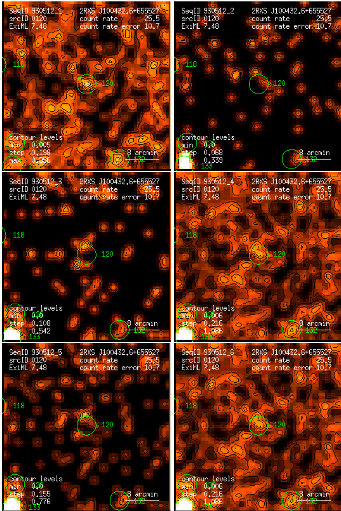
Figure 120: RASS 930512: detection 0120: band rate images, Gaussian filter: (1) PSPC channels 11 – 41, (2) 52 – 90, (3) 91 – 201, (4) 11 – 235, (5) 52 – 201, (6) 11 – 201. Broad band rates in counts/ks. Band rate contour levels in counts/ks/arcmin 2 .
