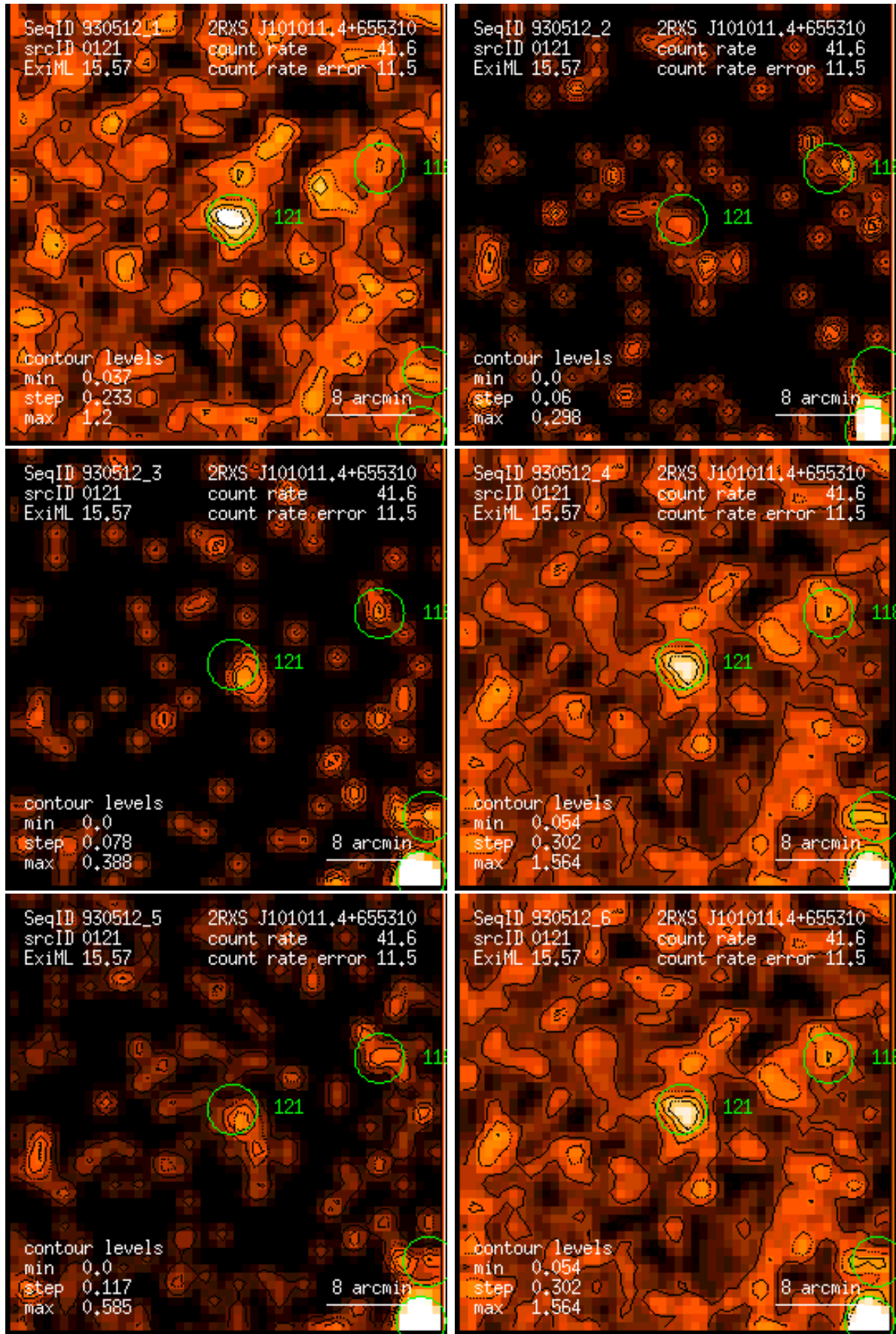
Figure 121: RASS 930512: detection 0121: band rate images, Gaussian filter: (1) PSPC channels 11 – 41, (2) 52 – 90, (3) 91 – 201, (4) 11 – 235, (5) 52 – 201, (6) 11 – 201. Broad band rates in counts/ks. Band rate contour levels in counts/ks/arcmin 2 .
