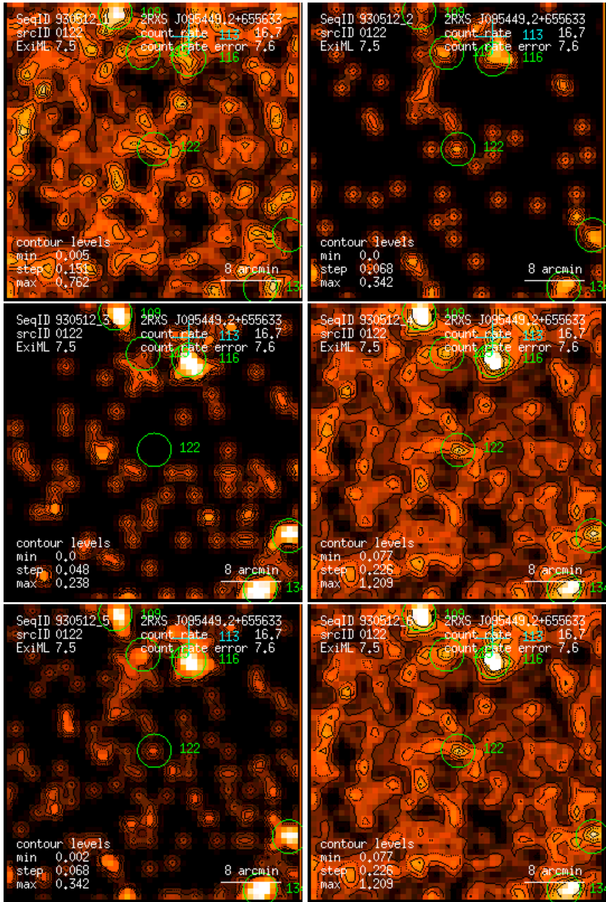
Figure 122: RASS 930512: detection 0122: band rate images, Gaussian filter: (1) PSPC channels 11 – 41, (2) 52 – 90, (3) 91 – 201, (4) 11 – 235, (5) 52 – 201, (6) 11 – 201. Broad band rates in counts/ks. Band rate contour levels in counts/ks/arcmin 2 .
