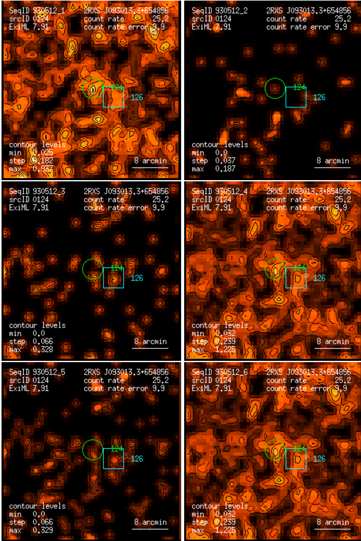
Figure 124: RASS 930512: detection 0124: band rate images, Gaussian filter: (1) PSPC channels 11 – 41, (2) 52 – 90, (3) 91 – 201, (4) 11 – 235, (5) 52 – 201, (6) 11 – 201. Broad band rates in counts/ks. Band rate contour levels in counts/ks/arcmin 2 .
