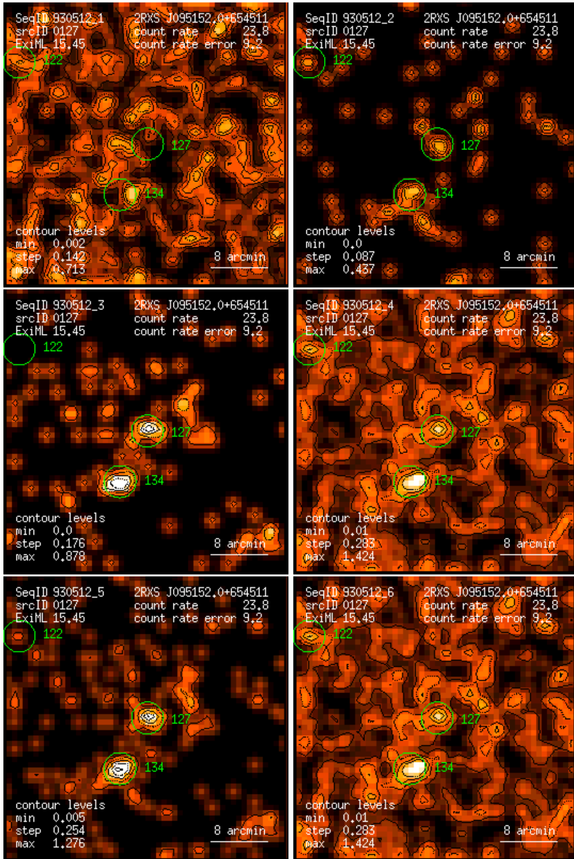
Figure 127: RASS 930512: detection 0127: band rate images, Gaussian filter: (1) PSPC channels 11 – 41, (2) 52 – 90, (3) 91 – 201, (4) 11 – 235, (5) 52 – 201, (6) 11 – 201. Broad band rates in counts/ks. Band rate contour levels in counts/ks/arcmin 2 .
