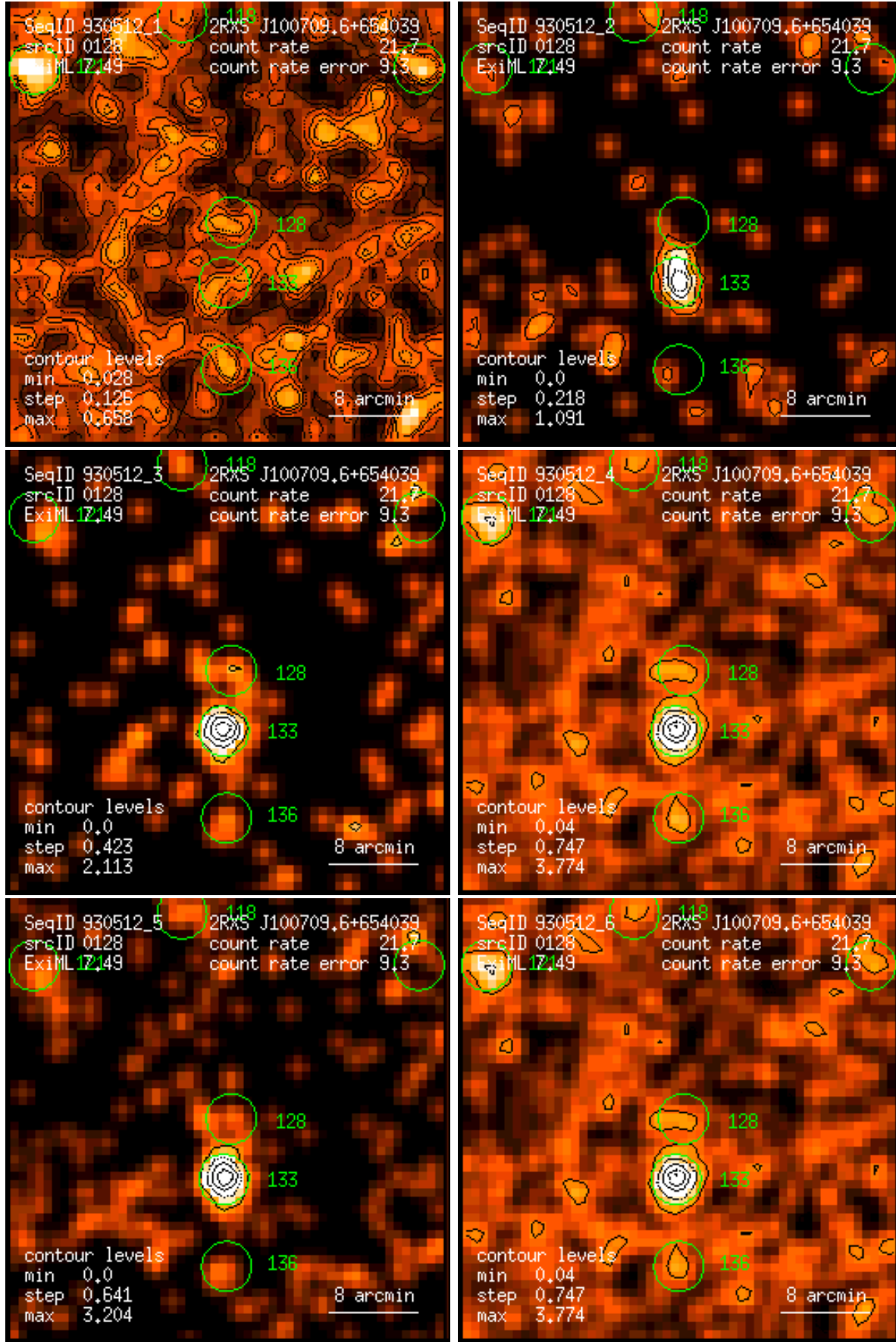
Figure 128: RASS 930512: detection 0128: band rate images, Gaussian filter: (1) PSPC channels 11 – 41, (2) 52 – 90, (3) 91 – 201, (4) 11 – 235, (5) 52 – 201, (6) 11 – 201. Broad band rates in counts/ks. Band rate contour levels in counts/ks/arcmin 2 .
