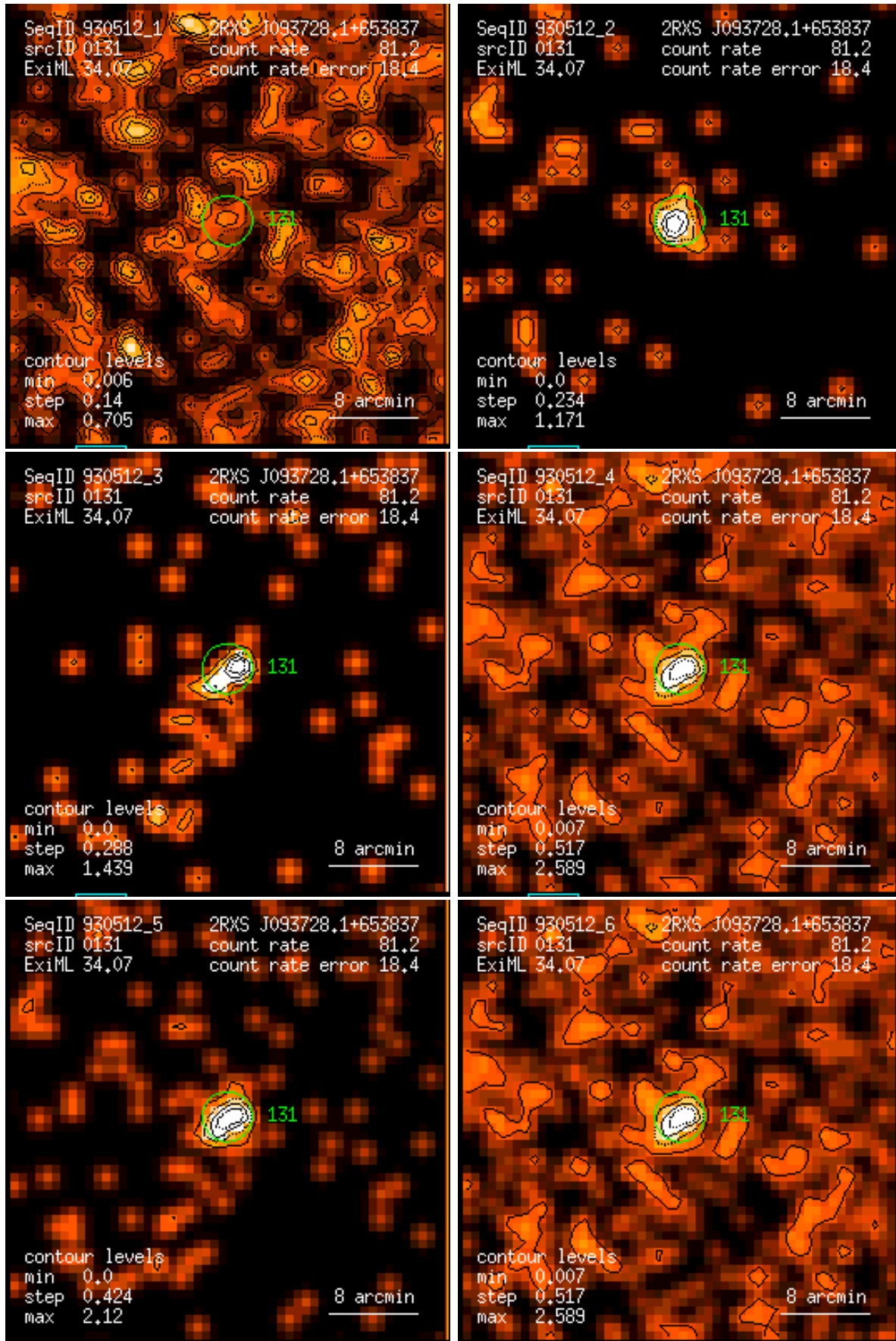
Figure 131: RASS 930512: detection 0131: band rate images, Gaussian filter: (1) PSPC channels 11 – 41, (2) 52 – 90, (3) 91 – 201, (4) 11 – 235, (5) 52 – 201, (6) 11 – 201. Broad band rates in counts/ks. Band rate contour levels in counts/ks/arcmin 2 .
