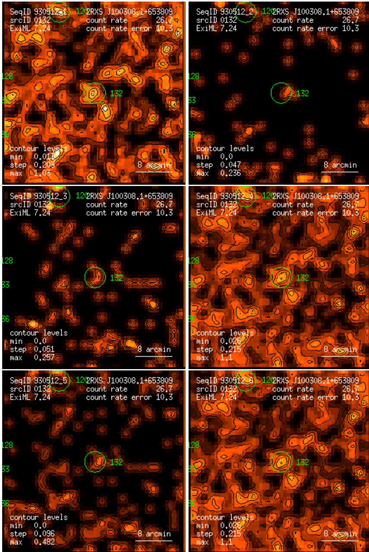
Figure 132: RASS 930512: detection 0132: band rate images, Gaussian filter: (1) PSPC channels 11 – 41, (2) 52 – 90, (3) 91 – 201, (4) 11 – 235, (5) 52 – 201, (6) 11 – 201. Broad band rates in counts/ks. Band rate contour levels in counts/ks/arcmin 2 .
