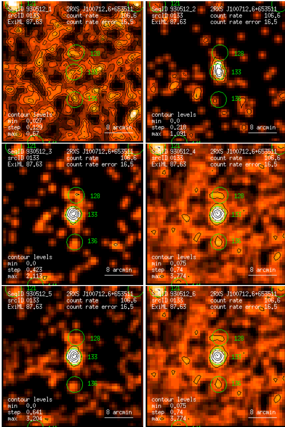
Figure 133: RASS 930512: detection 0133: band rate images, Gaussian filter: (1) PSPC channels 11 – 41, (2) 52 – 90, (3) 91 – 201, (4) 11 – 235, (5) 52 – 201, (6) 11 – 201. Broad band rates in counts/ks. Band rate contour levels in counts/ks/arcmin 2 .
