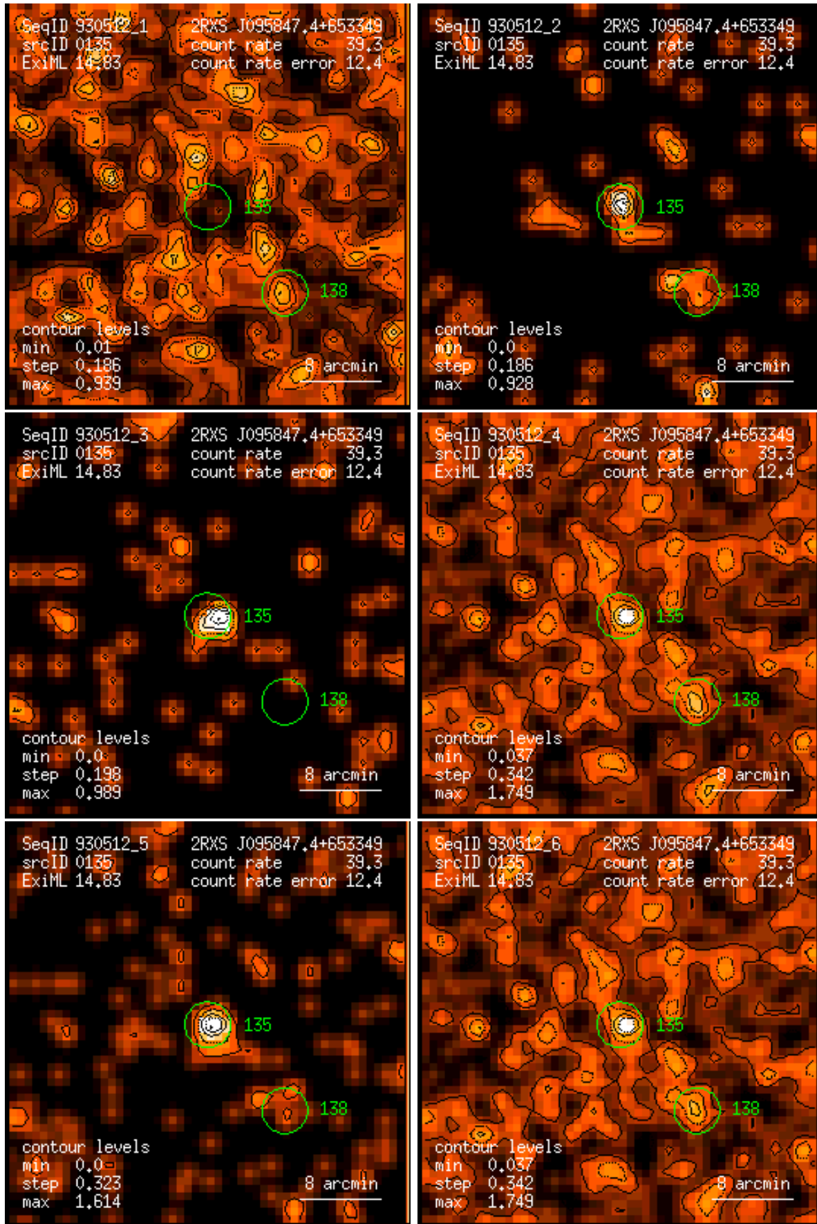
Figure 135: RASS 930512: detection 0135: band rate images, Gaussian filter: (1) PSPC channels 11 – 41, (2) 52 – 90, (3) 91 – 201, (4) 11 – 235, (5) 52 – 201, (6) 11 – 201. Broad band rates in counts/ks. Band rate contour levels in counts/ks/arcmin 2 .
