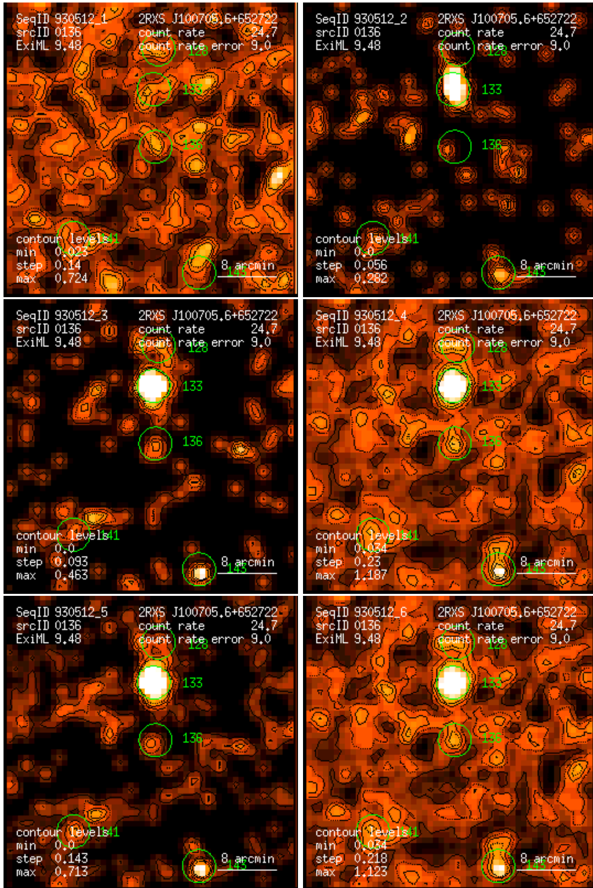
Figure 136: RASS 930512: detection 0136: band rate images, Gaussian filter: (1) PSPC channels 11 – 41, (2) 52 – 90, (3) 91 – 201, (4) 11 – 235, (5) 52 – 201, (6) 11 – 201. Broad band rates in counts/ks. Band rate contour levels in counts/ks/arcmin 2 .
