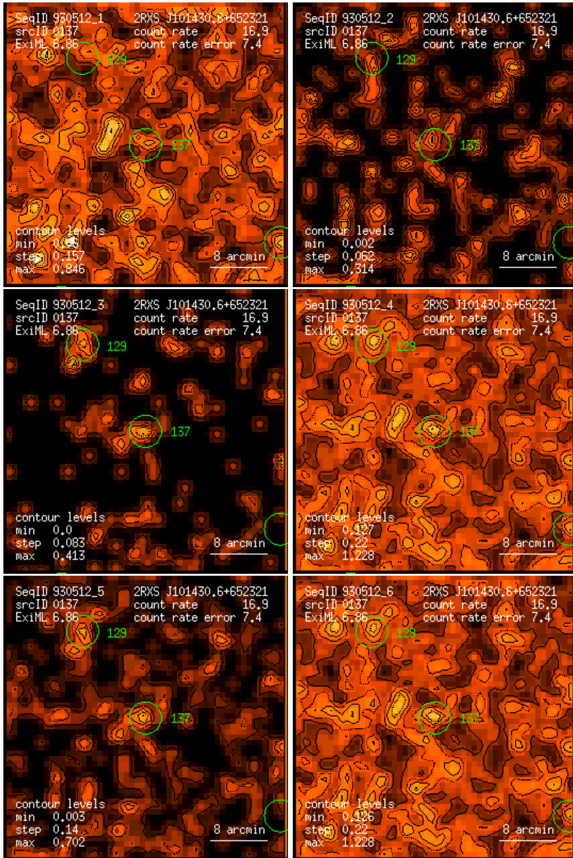
Figure 137: RASS 930512: detection 0137: band rate images, Gaussian filter: (1) PSPC channels 11 – 41, (2) 52 – 90, (3) 91 – 201, (4) 11 – 235, (5) 52 – 201, (6) 11 – 201. Broad band rates in counts/ks. Band rate contour levels in counts/ks/arcmin 2 .
