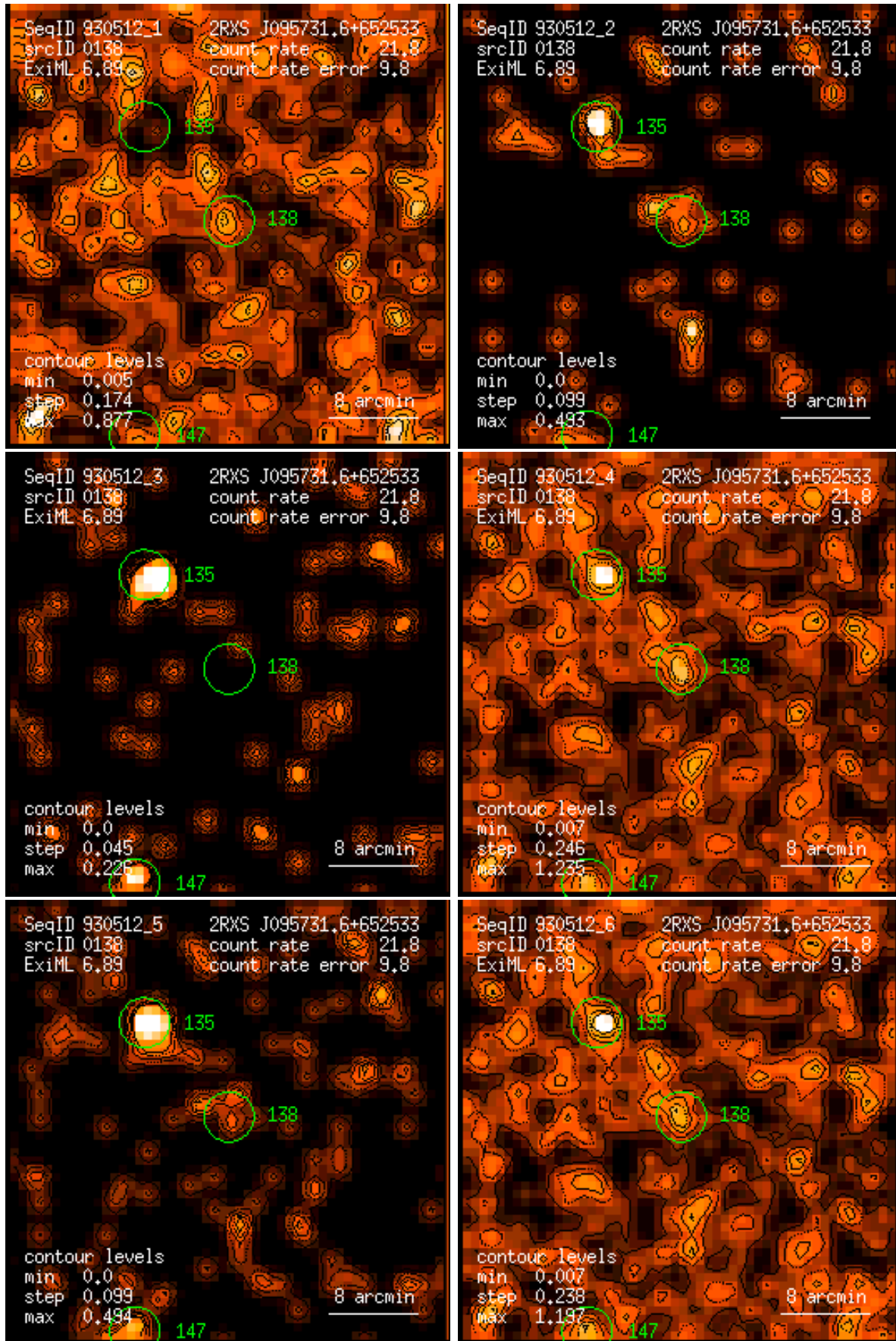
Figure 138: RASS 930512: detection 0138: band rate images, Gaussian filter: (1) PSPC channels 11 – 41, (2) 52 – 90, (3) 91 – 201, (4) 11 – 235, (5) 52 – 201, (6) 11 – 201. Broad band rates in counts/ks. Band rate contour levels in counts/ks/arcmin 2 .
