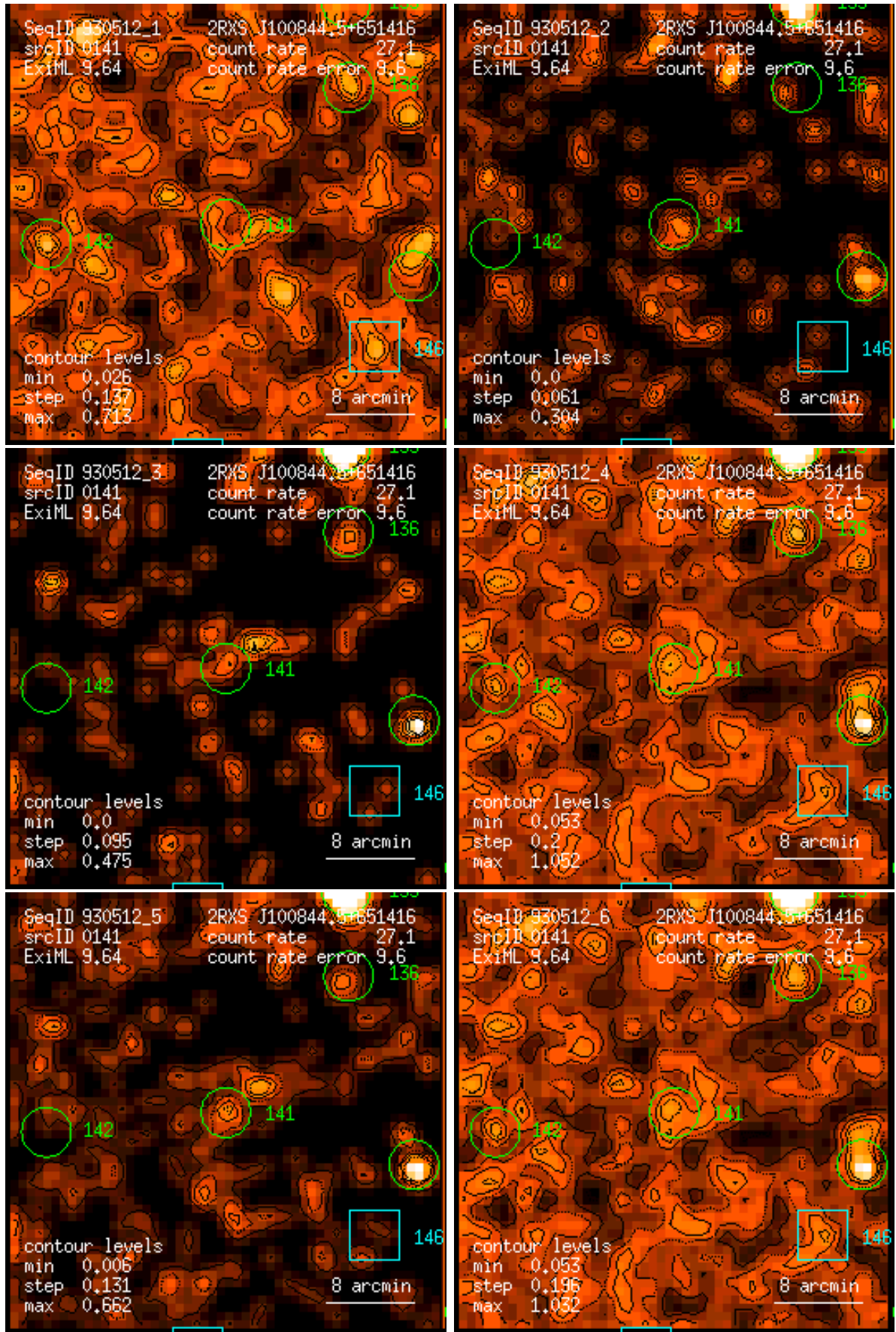
Figure 141: RASS 930512: detection 0141: band rate images, Gaussian filter: (1) PSPC channels 11 – 41, (2) 52 – 90, (3) 91 – 201, (4) 11 – 235, (5) 52 – 201, (6) 11 – 201. Broad band rates in counts/ks. Band rate contour levels in counts/ks/arcmin 2 .
