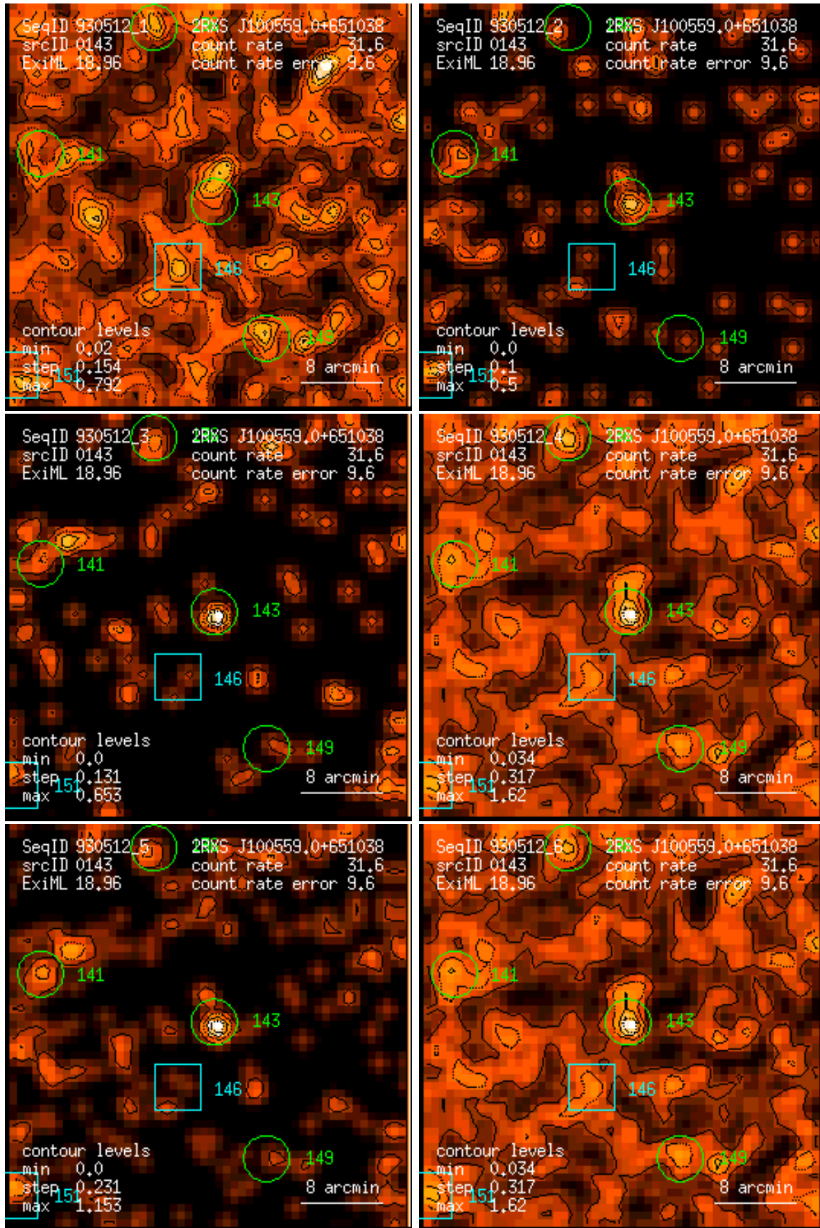
Figure 143: RASS 930512: detection 0143: band rate images, Gaussian filter: (1) PSPC channels 11 – 41, (2) 52 – 90, (3) 91 – 201, (4) 11 – 235, (5) 52 – 201, (6) 11 – 201. Broad band rates in counts/ks. Band rate contour levels in counts/ks/arcmin 2 .
