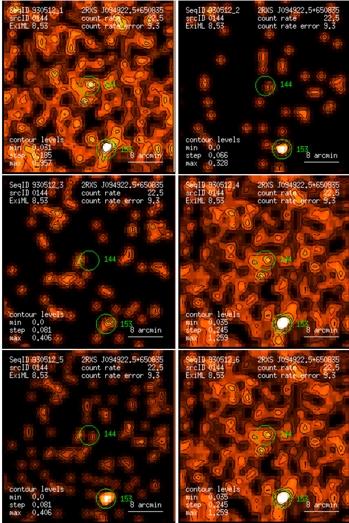
Figure 144: RASS 930512: detection 0144: band rate images, Gaussian filter: (1) PSPC channels 11 – 41, (2) 52 – 90, (3) 91 – 201, (4) 11 – 235, (5) 52 – 201, (6) 11 – 201. Broad band rates in counts/ks. Band rate contour levels in counts/ks/arcmin 2 .
