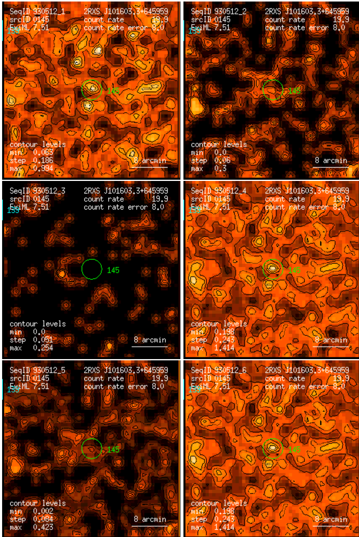
Figure 145: RASS 930512: detection 0145: band rate images, Gaussian filter: (1) PSPC channels 11 – 41, (2) 52 – 90, (3) 91 – 201, (4) 11 – 235, (5) 52 – 201, (6) 11 – 201. Broad band rates in counts/ks. Band rate contour levels in counts/ks/arcmin 2 .
