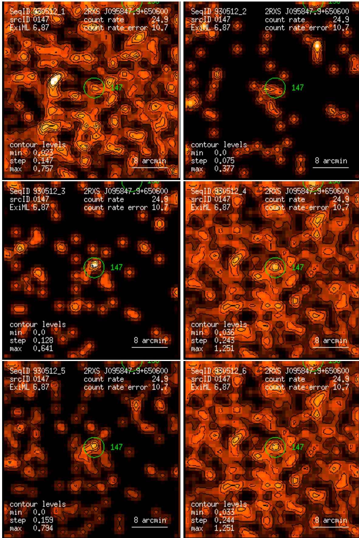
Figure 147: RASS 930512: detection 0147: band rate images, Gaussian filter: (1) PSPC channels 11 – 41, (2) 52 – 90, (3) 91 – 201, (4) 11 – 235, (5) 52 – 201, (6) 11 – 201. Broad band rates in counts/ks. Band rate contour levels in counts/ks/arcmin 2 .
