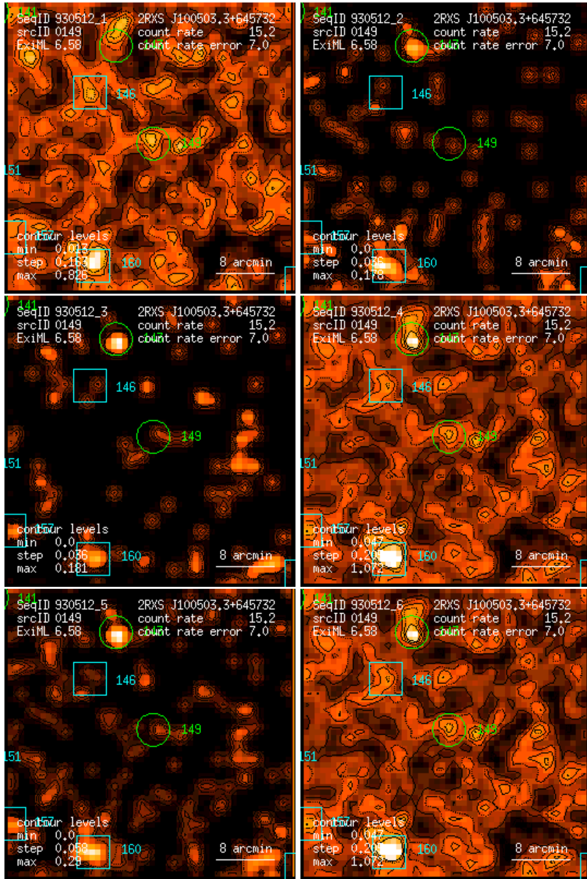
Figure 149: RASS 930512: detection 0149: band rate images, Gaussian filter: (1) PSPC channels 11 – 41, (2) 52 – 90, (3) 91 – 201, (4) 11 – 235, (5) 52 – 201, (6) 11 – 201. Broad band rates in counts/ks. Band rate contour levels in counts/ks/arcmin 2 .
