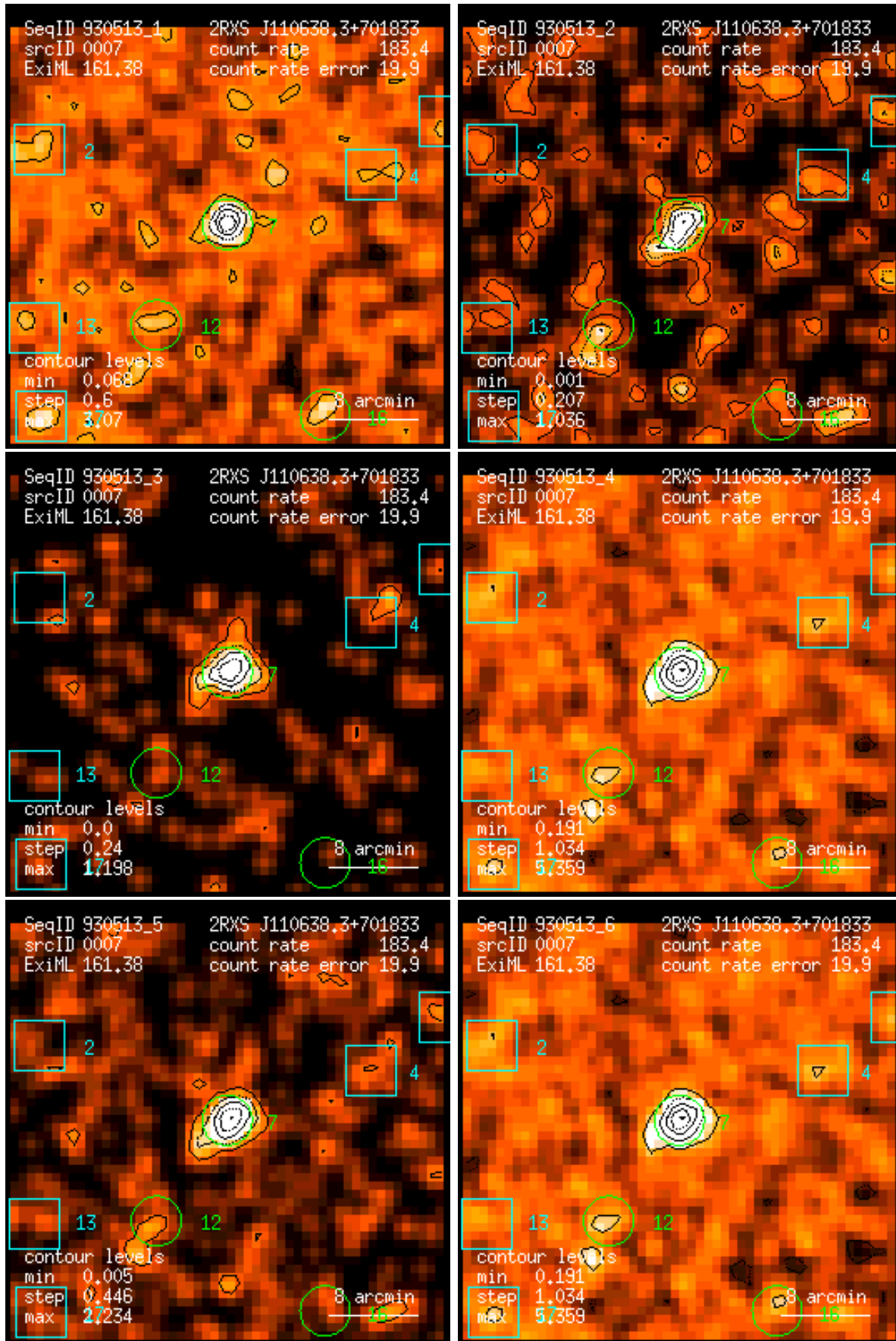
Figure 7: RASS 930513: detection 0007: band rate images, Gaussian filter: (1) PSPC channels 11 – 41, (2) 52 – 90, (3) 91 – 201, (4) 11 – 235, (5) 52 – 201, (6) 11 – 201. Broad band rates in counts/ks. Band rate contour levels in counts/ks/arcmin 2 .
