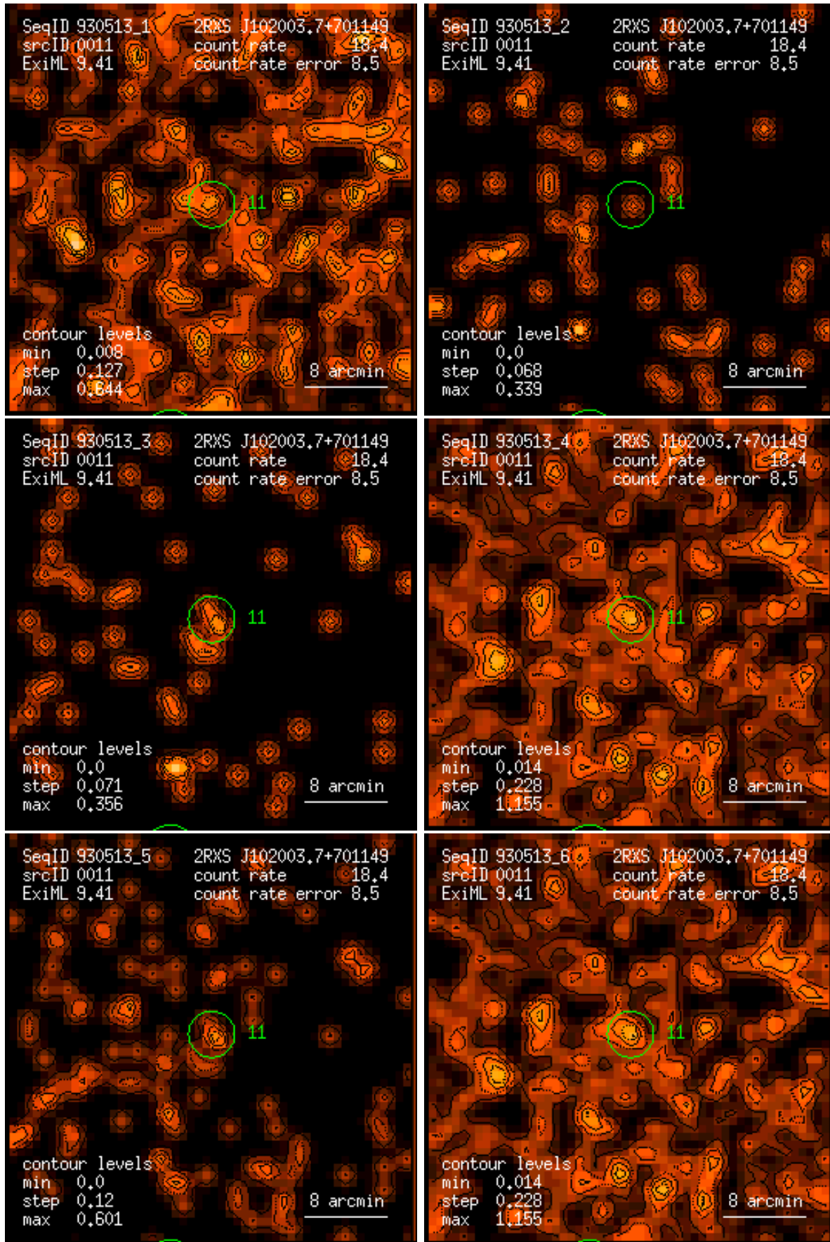
Figure 11: RASS 930513: detection 0011: band rate images, Gaussian filter: (1) PSPC channels 11 – 41, (2) 52 – 90, (3) 91 – 201, (4) 11 – 235, (5) 52 – 201, (6) 11 – 201. Broad band rates in counts/ks. Band rate contour levels in counts/ks/arcmin 2 .
