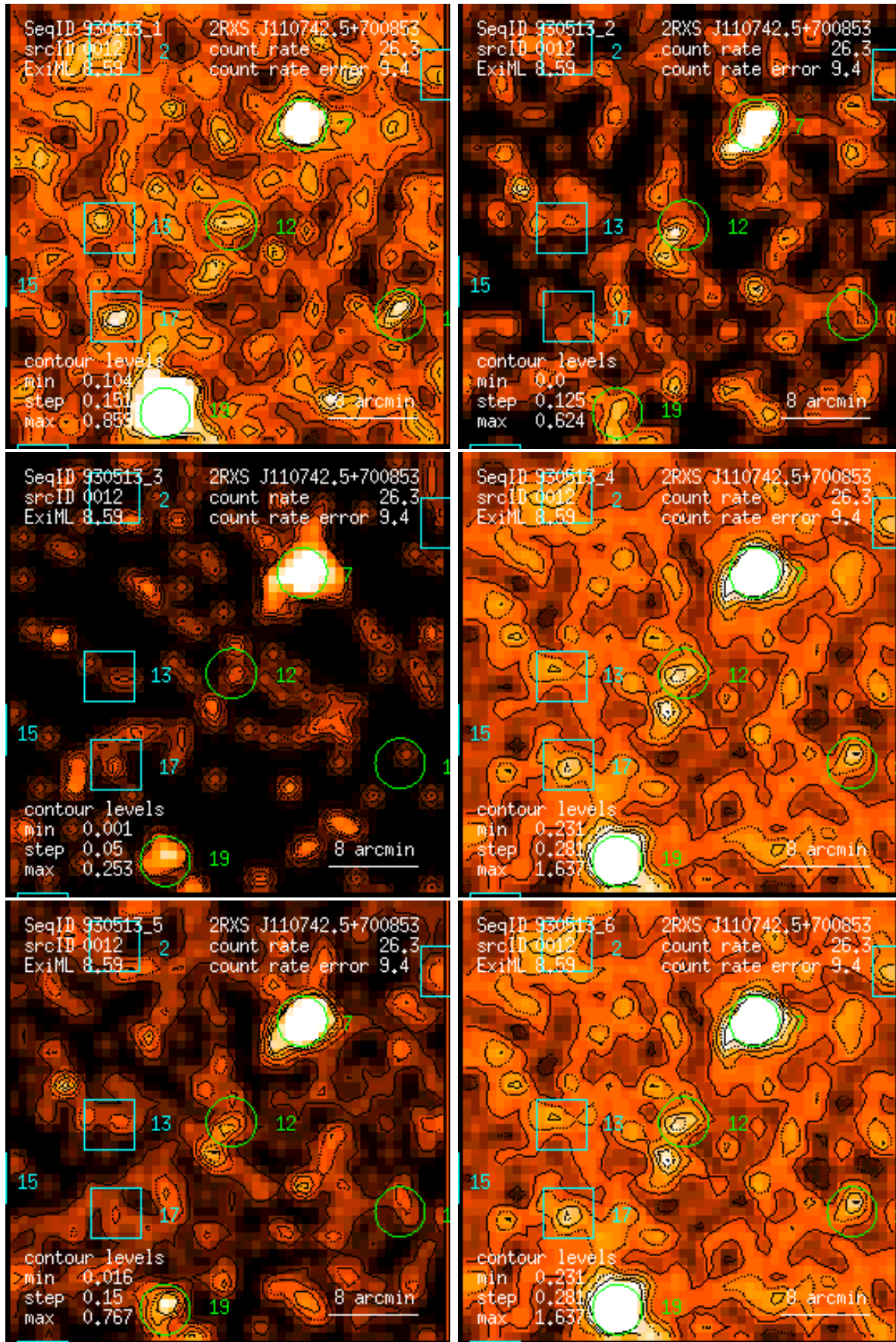
Figure 12: RASS 930513: detection 0012: band rate images, Gaussian filter: (1) PSPC channels 11 – 41, (2) 52 – 90, (3) 91 – 201, (4) 11 – 235, (5) 52 – 201, (6) 11 – 201. Broad band rates in counts/ks. Band rate contour levels in counts/ks/arcmin 2 .
