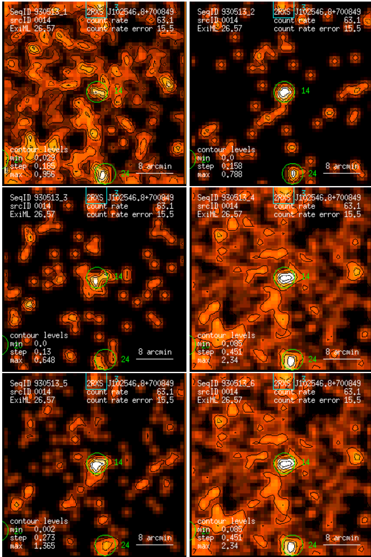
Figure 14: RASS 930513: detection 0014: band rate images, Gaussian filter: (1) PSPC channels 11 – 41, (2) 52 – 90, (3) 91 – 201, (4) 11 – 235, (5) 52 – 201, (6) 11 – 201. Broad band rates in counts/ks. Band rate contour levels in counts/ks/arcmin 2 .
