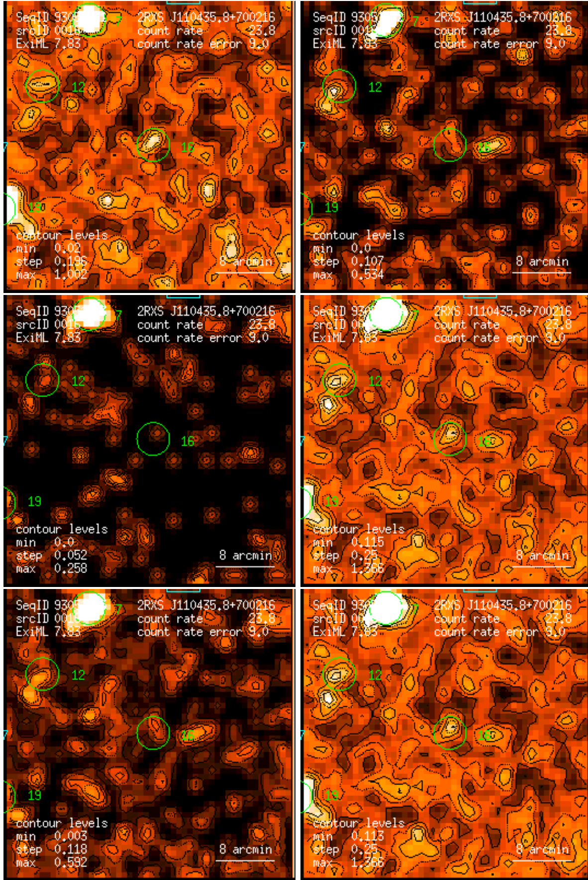
Figure 16: RASS 930513: detection 0016: band rate images, Gaussian filter: (1) PSPC channels 11 – 41, (2) 52 – 90, (3) 91 – 201, (4) 11 – 235, (5) 52 – 201, (6) 11 – 201. Broad band rates in counts/ks. Band rate contour levels in counts/ks/arcmin 2 .
