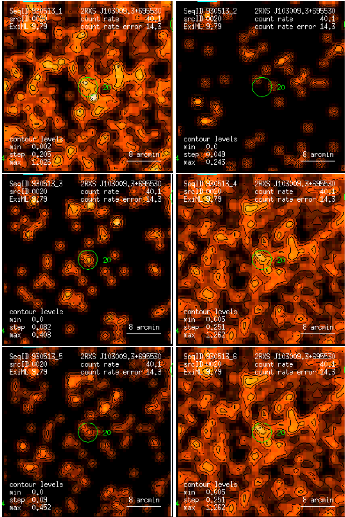
Figure 20: RASS 930513: detection 0020: band rate images, Gaussian filter: (1) PSPC channels 11 – 41, (2) 52 – 90, (3) 91 – 201, (4) 11 – 235, (5) 52 – 201, (6) 11 – 201. Broad band rates in counts/ks. Band rate contour levels in counts/ks/arcmin 2 .
