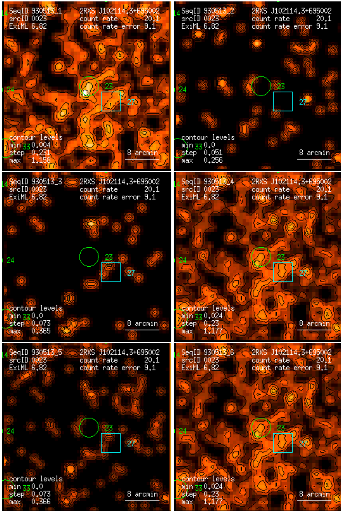
Figure 23: RASS 930513: detection 0023: band rate images, Gaussian filter: (1) PSPC channels 11 – 41, (2) 52 – 90, (3) 91 – 201, (4) 11 – 235, (5) 52 – 201, (6) 11 – 201. Broad band rates in counts/ks. Band rate contour levels in counts/ks/arcmin 2 .
