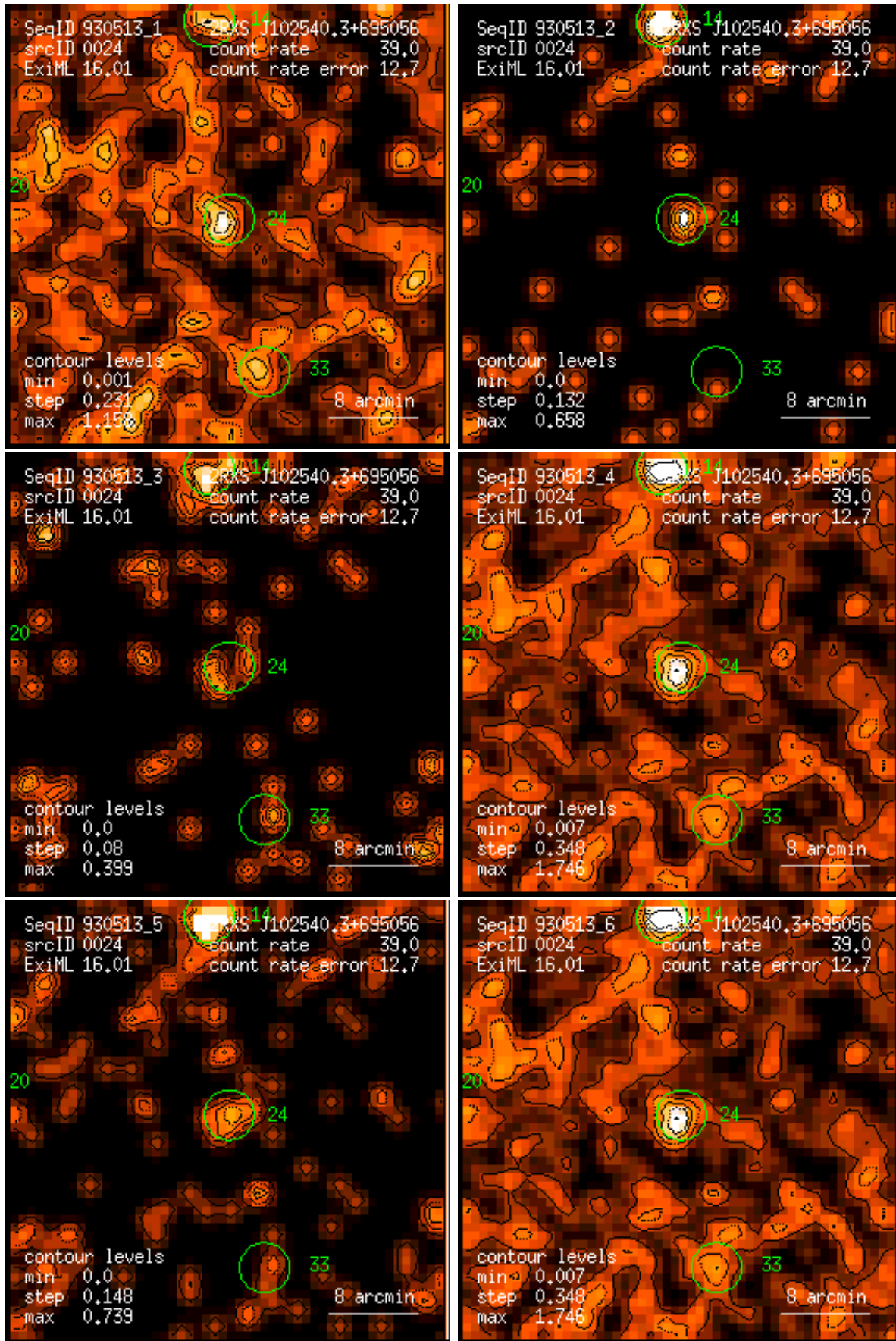
Figure 24: RASS 930513: detection 0024: band rate images, Gaussian filter: (1) PSPC channels 11 – 41, (2) 52 – 90, (3) 91 – 201, (4) 11 – 235, (5) 52 – 201, (6) 11 – 201. Broad band rates in counts/ks. Band rate contour levels in counts/ks/arcmin 2 .
