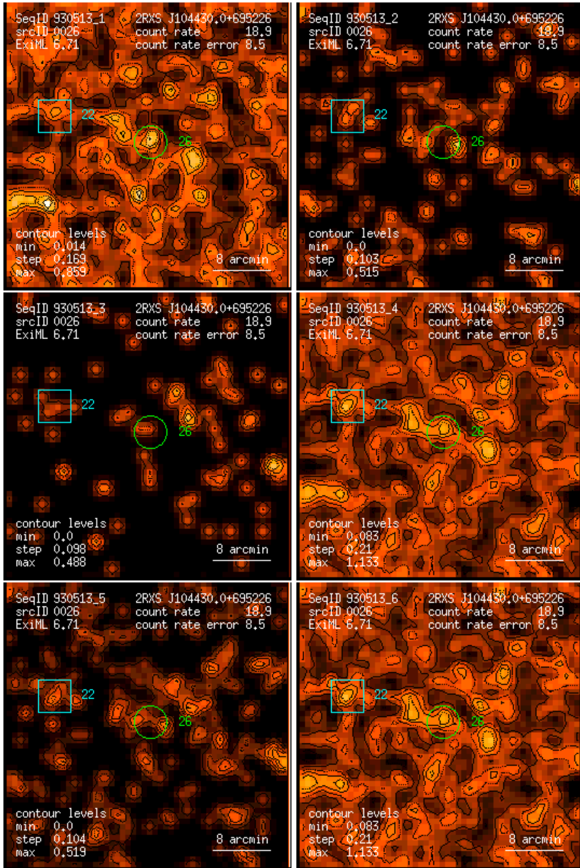
Figure 26: RASS 930513: detection 0026: band rate images, Gaussian filter: (1) PSPC channels 11 – 41, (2) 52 – 90, (3) 91 – 201, (4) 11 – 235, (5) 52 – 201, (6) 11 – 201. Broad band rates in counts/ks. Band rate contour levels in counts/ks/arcmin 2 .
