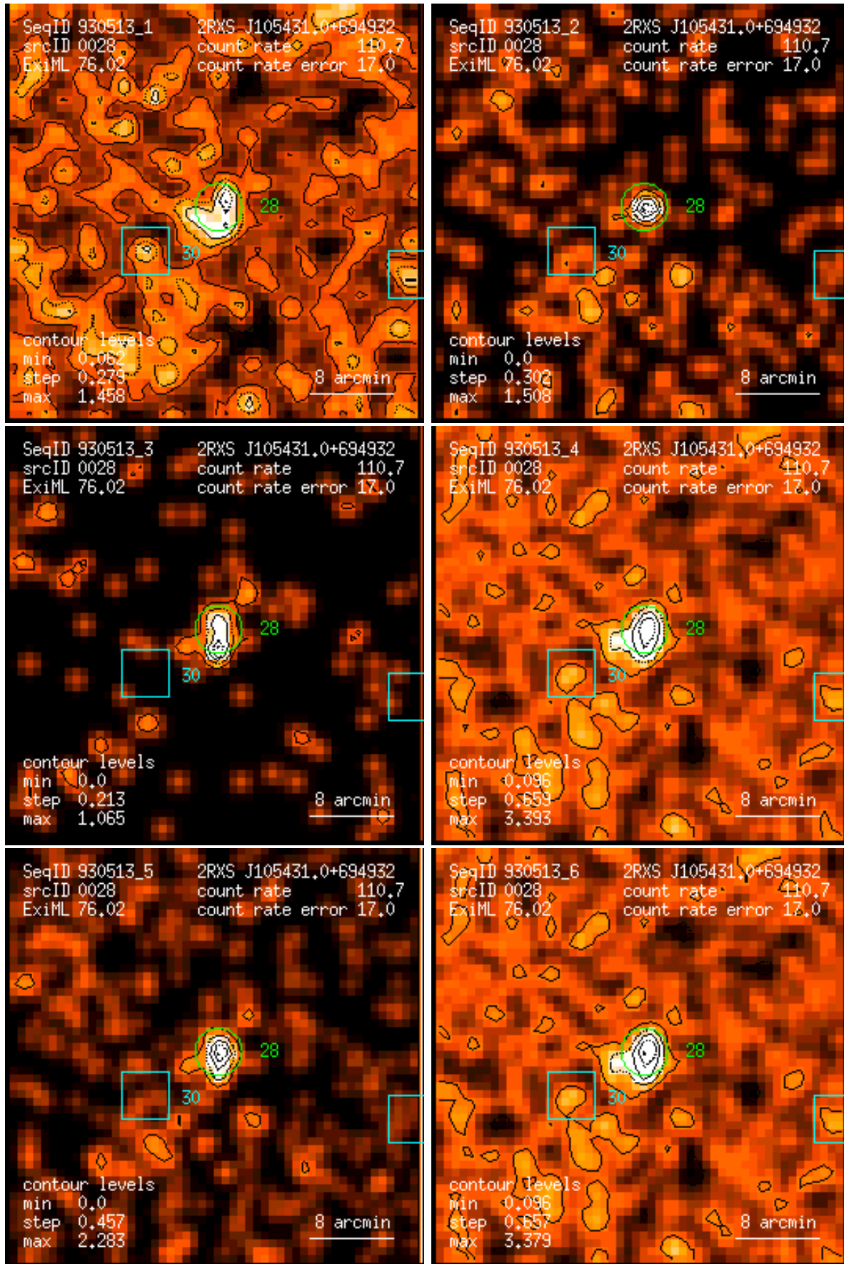
Figure 28: RASS 930513: detection 0028: band rate images, Gaussian filter: (1) PSPC channels 11 – 41, (2) 52 – 90, (3) 91 – 201, (4) 11 – 235, (5) 52 – 201, (6) 11 – 201. Broad band rates in counts/ks. Band rate contour levels in counts/ks/arcmin 2 .
