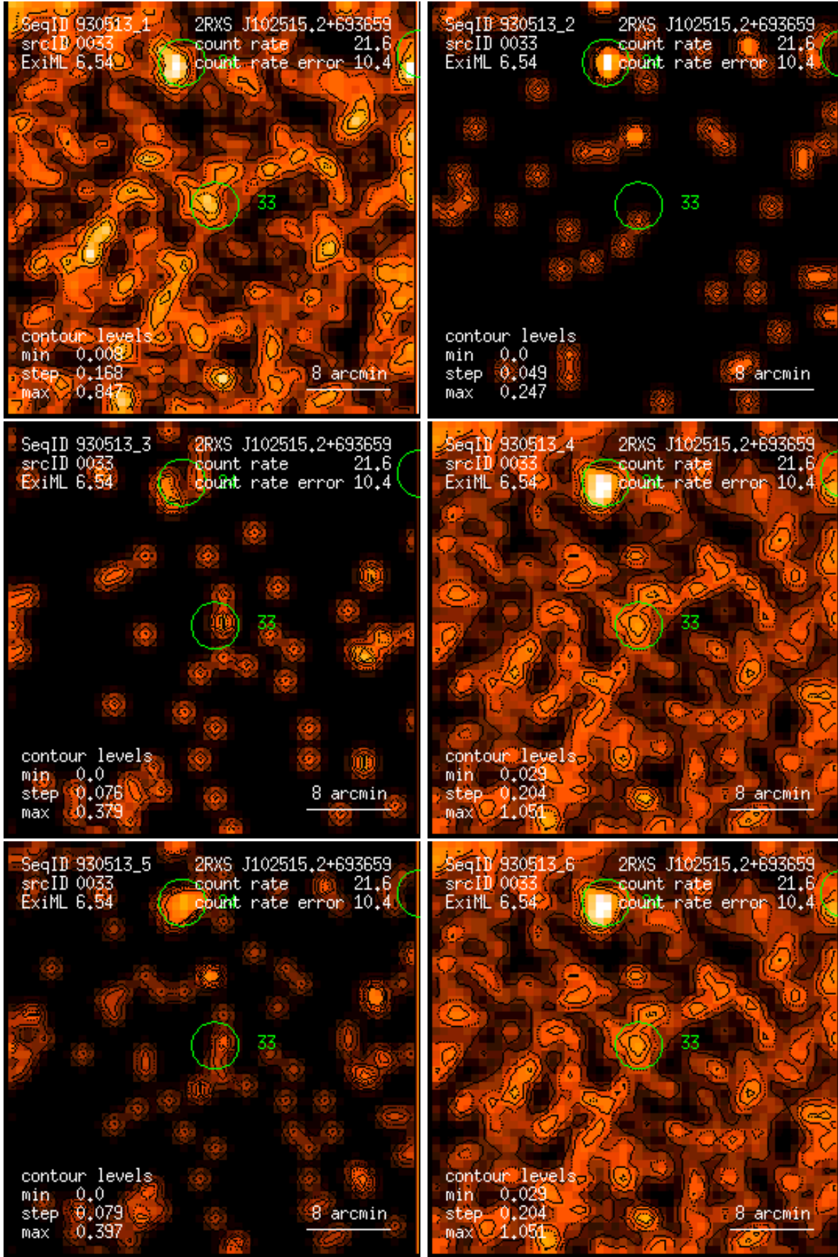
Figure 33: RASS 930513: detection 0033: band rate images, Gaussian filter: (1) PSPC channels 11 – 41, (2) 52 – 90, (3) 91 – 201, (4) 11 – 235, (5) 52 – 201, (6) 11 – 201. Broad band rates in counts/ks. Band rate contour levels in counts/ks/arcmin 2 .
